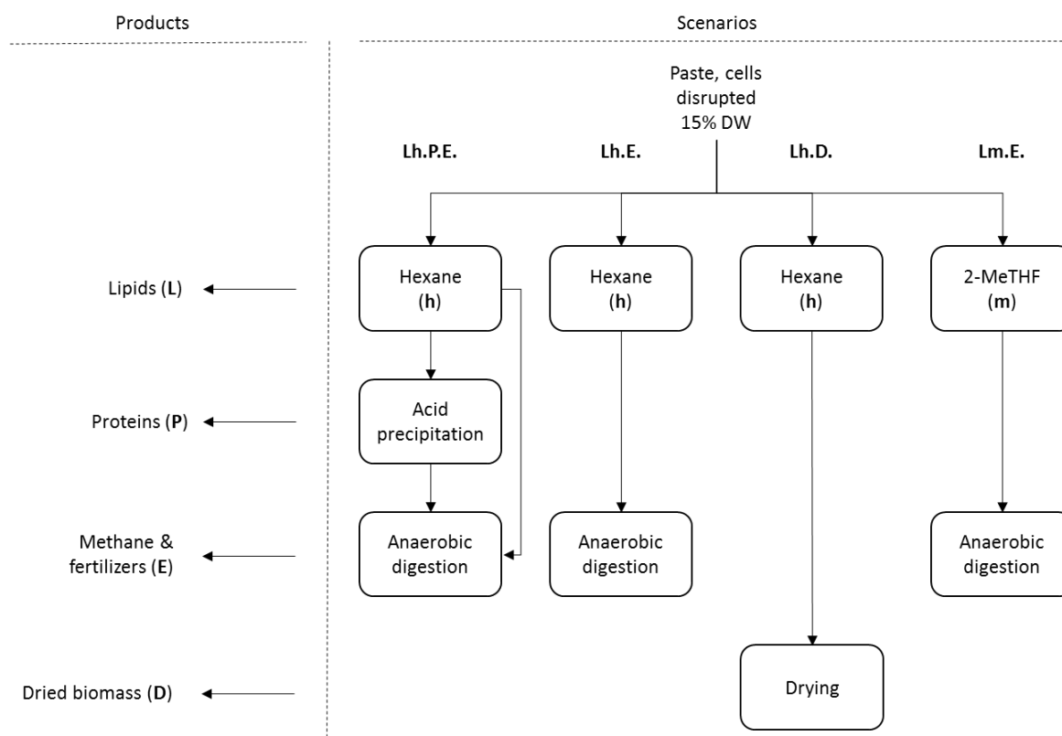
Figure 4- 1 Biorefinery scenarios for microalgae wet biomass valorisation. Lh.P.E.: hexane lipid extraction, proteins extraction, energy production; Lh.E.: hexane lipid extraction, energy production; Lh.D.: hexane lipid extraction, dried biomass production; Lm.E. 2-Methyltetrahydrofuran lipid extraction, energy production; DW: dry weight. For each scenario, two methods for cells disruption are tested: bead mill (BM) and high-pressure homogenisation (HPH) (c.f. 4.2.3.2).
