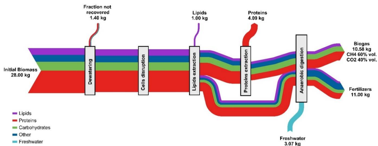
Figure 4- 2 Fate of the constituents of Chlorella vulgaris within the hexane lipid extraction, proteins extraction, anaerobic digestion scenario (Lh.P.E.) to extract 1 kilogram of lipids. Biomass composition is expressed in kilogram [kg] of dried weight.
