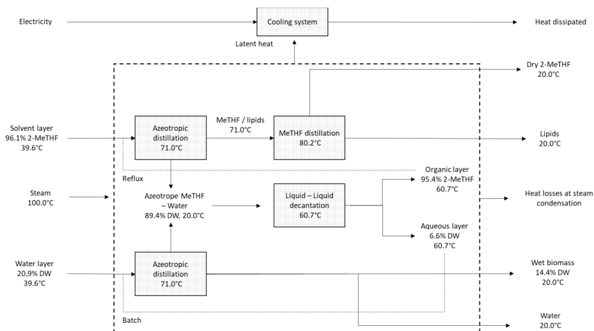
Figure B- 2 Generic flow diagram for the recovery of dry 2-MeTHF via continuous azeotropic distillation and the recovery of lipids via 2-MeTHF distillation.
