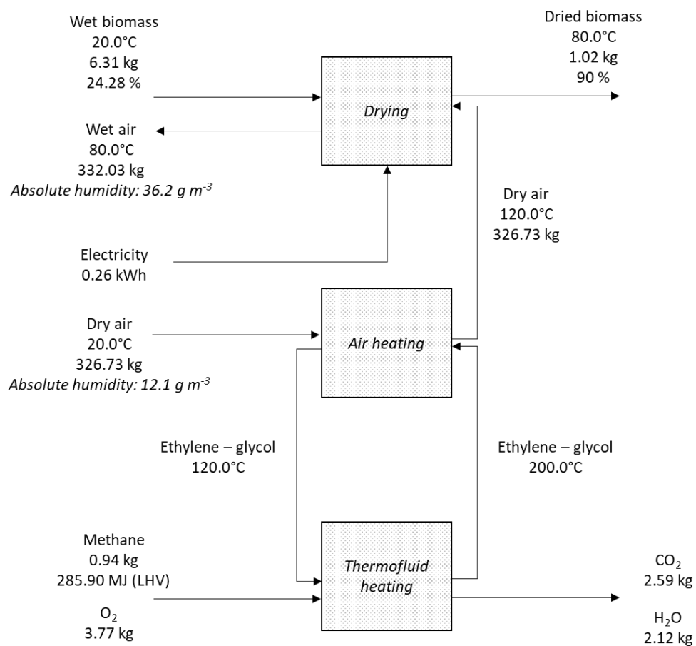
Figure B- 5 Mass and energy flows diagram for drying algae wet biomass resulting from hexane lipid extraction. Values are reported per kg dry weight at the biorefinery gate, heat losses are not shown.
