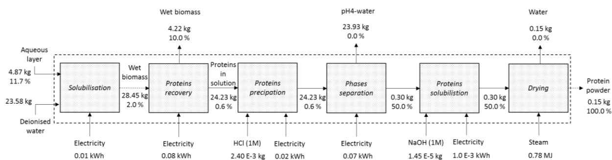
Figure B- 3 Mass and energy flows diagram for proteins extraction from waste biomass resulting from hexane lipid extraction. Values are reported per kg dry weight at the biorefinery gate, heat losses are not shown.
