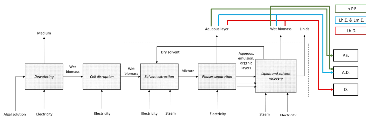
Figure B- 1 Generic flow diagram for pre-extraction steps and lipid extraction applicable for all scenarios. Detailed values for mass and energy flows are provided in Table 1 and Table 2. The lipid extraction step is delimited by dotted lines. The coloured arrows represent the fate of the streams to further valorisation steps according to the scenario (P.E. Proteins Extraction, A.D. Anaerobic Digestion, D. Drying biomass).
