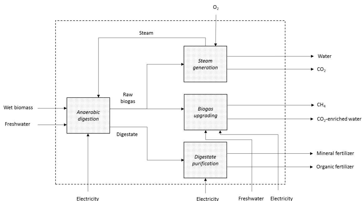
Figure B- 4 Generic flow diagram for anaerobic digestion step. Detailed values for mass and energy flows are provided in Table 4.
