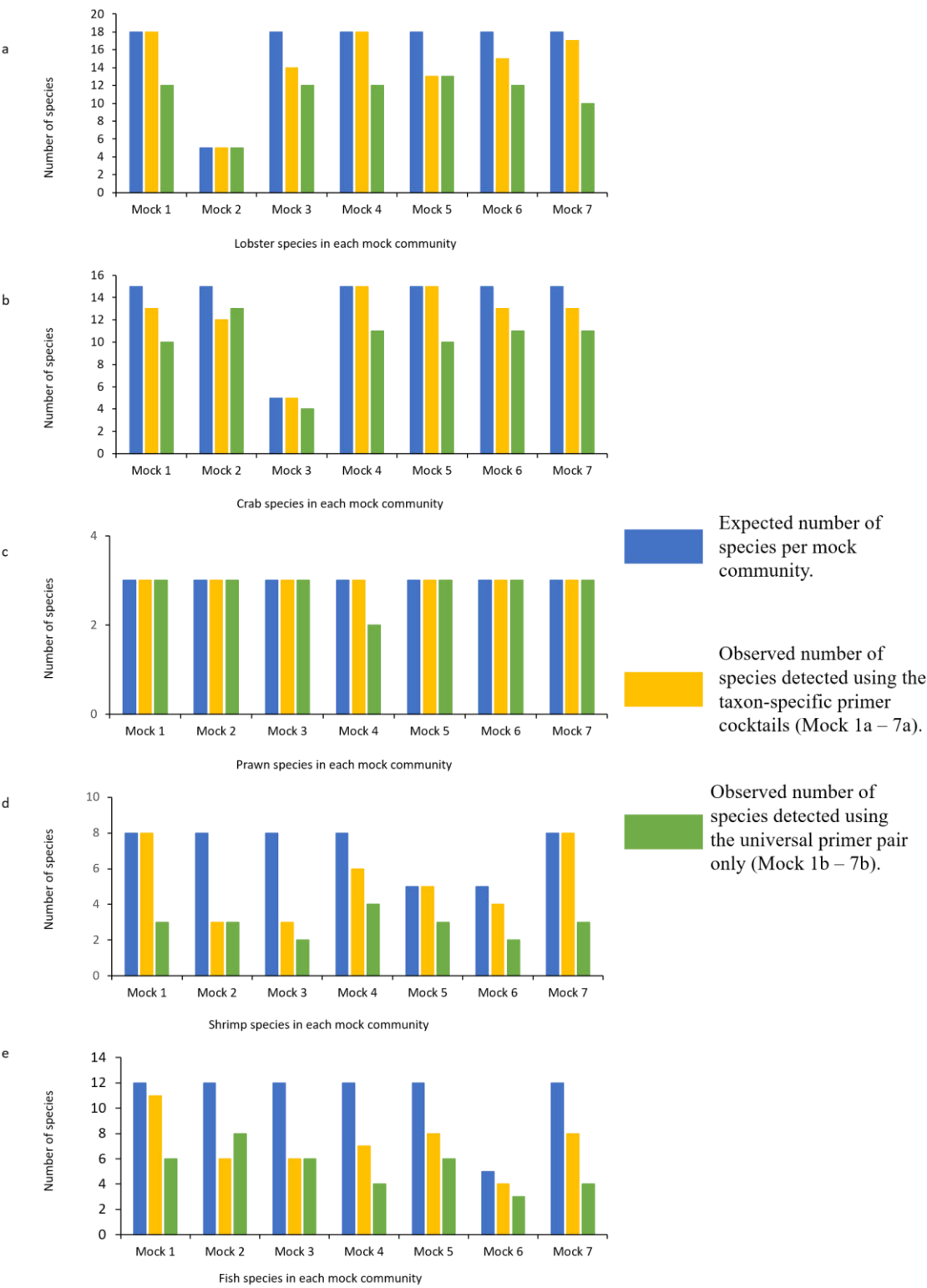
3 4 Figure 3.2 The expected number of species vs. the observed number of species for each taxonomic group in 5 each mock community.
