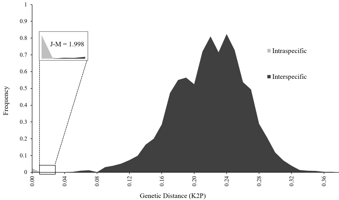
Figure 2.1 Frequency distributions of intra- and interspecific pairwise K2P distances calculated using the selected mini-barcode region (Fragment 230_b). The barcode gap (insert) lies between the genetic distances of 0.01 and 0.02.
