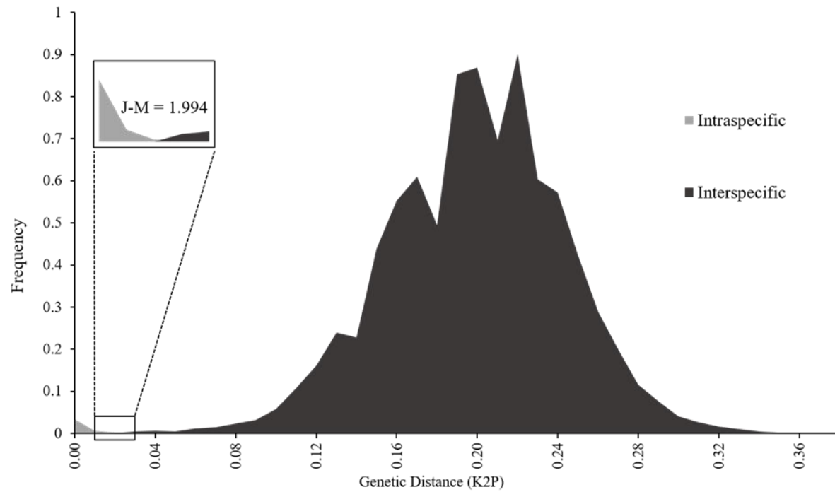
Figure S2.2 Frequency distribution of intra- and interspecific pairwise K2P distances calculated using the selected mini-barcode region (Fragment 230_b). The barcode gap (insert) lies between the genetic distances of 0.02 and 0.03.
