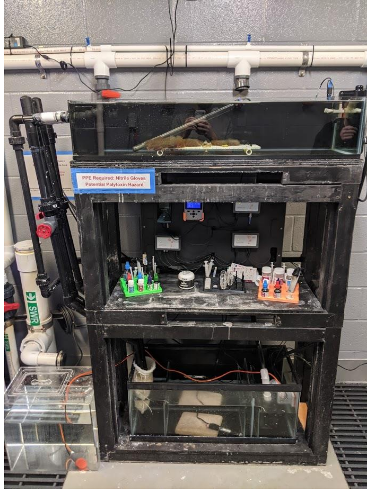
Figure 2.2: Coral tank set up. Top tank held the coral, probes, 300-watt heater, and UV sterilizer. Bottom middle tank is the sub tank. This tank held two 50-watt heaters, a sock, bio substrate and auto top off output. Left bottom tank was the top off tank that holds the auto top off intake.
