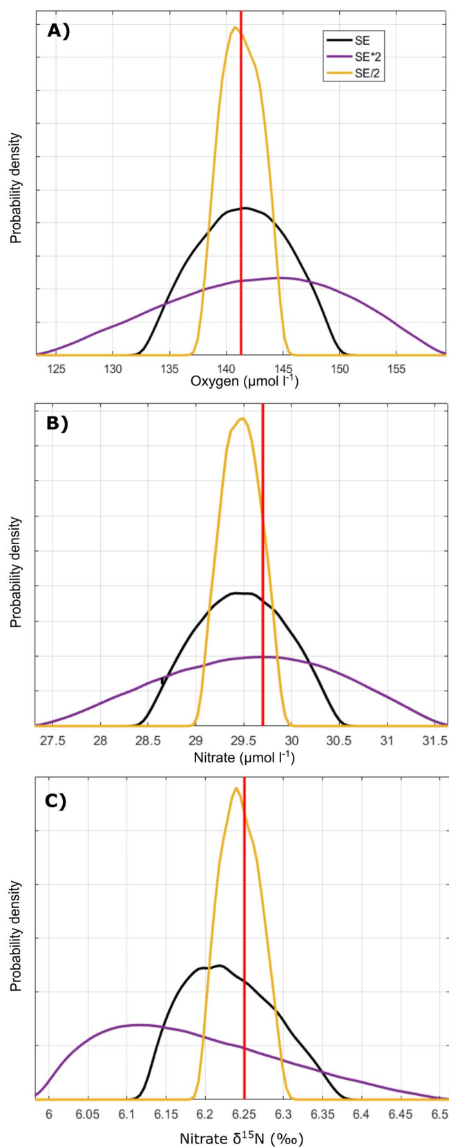
Extended Data Fig. 6 | Probability density function of the model best fits for O_2 concentration, NO_3^- concentration, and NO_3^- \delta^{15}N . The colors represent different choices for the standard error: SE = standard error in the standard run (black line); SE*2 = 2 times higher standard error (purple line); and SE/2 = 2 times lower standard error (orange line). The vertical red bars indicate the corresponding mean weighted pycnocline values from the observations (Table 1).
