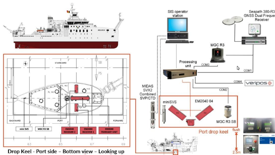
Figure 1. The new RV Belgica EM2040 dual Rx shallow water multibeam echosounder.
