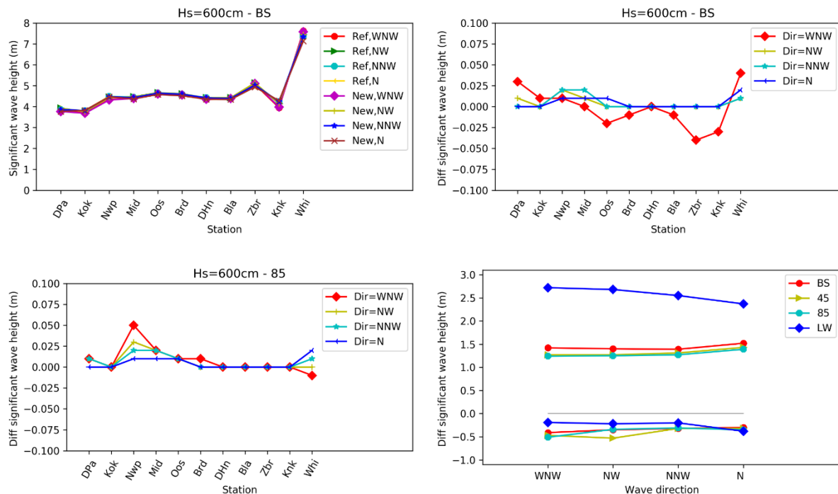
Figure 7: Upper left: Significant wave height at coastal stations and Westhinder for simulation with the new proposed extraction limit (New) compared to without extraction (Ref). Waves at boundary with significant wave height of 6.0 m, wind speed = 30 m/s, water level at 4.67 m MSL (1000 yearly storm). Results for different wave and wind directions. Upper right: Increase of significant wave height at coastal stations and Westhinder for simulation with the proposed extraction limit compared to without extraction, water level at 4.67 m MSL. Lower left: Increase of significant wave height at coastal stations and Westhinder for simulation with the proposed extraction limit compared to without extraction, water level at 5.52 m MSL (1000 yearly storm + sea level rise RCP 8.5).
