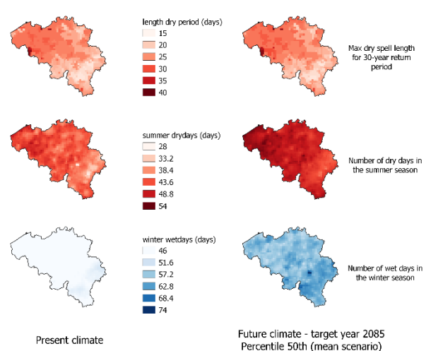
Figure 3 Mean impacts on the rainfall occurrence for the summer and the winter seasons. At the top the max length of the dry spells for a 30-year return period, in the middle the dry day frequency in the summer, and at the bottom the wet day frequency in the winter
