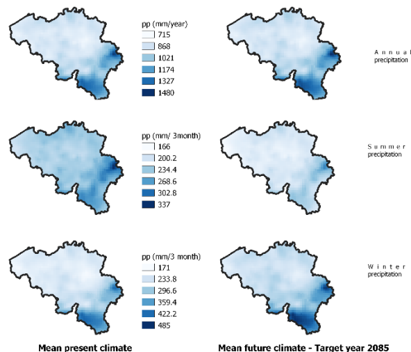
Figure 2 Mean impacts on the rainfall amounts for different aggregation levels; at the top the annual rainfall, in the middle the summer rainfall, and at the bottom, the winter rainfall. Present conditions are on the left and future conditions on the right.
