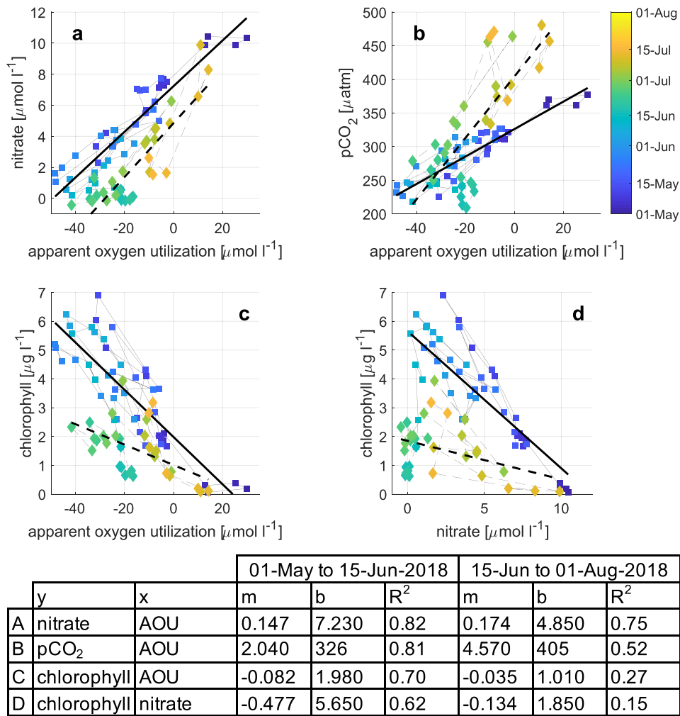
Fig. 7 Stoichiometry of bloom in mixed layer regime. Scatter plots of daily averages of apparent oxygen utilization (AOU) [ \mu\text{mol l}^{-1} ], nitrate [ \mu\text{mol l}^{-1} ], pCO 2 [ \mu\text{atm} ], and chlorophyll [ \mu\text{g l}^{-1} ] colored by date in 2018 at HG-IV. a Nitrate vs. AOU, b pCO 2 vs. AOU, c chlorophyll vs. AOU, and d chlorophyll vs. nitrate. Colored squares are data between 01-May-2018 and 15-Jun-2018 during the spring bloom. The squares are connected by gray solid lines. A least-squares regression curve is plotted as a solid black line for the time period and the regressions' parameters for the model y = m \times x + b are given in the table at the bottom for the different parameter relations and time periods. Colored diamonds/dashed lines are the same for the time period after the bloom (15-Jun-2018 to 01-Aug-2018). Note that this analysis could not be done in 2017 as the observations were below the productive layer and no nitrate and chlorophyll observations exist.
