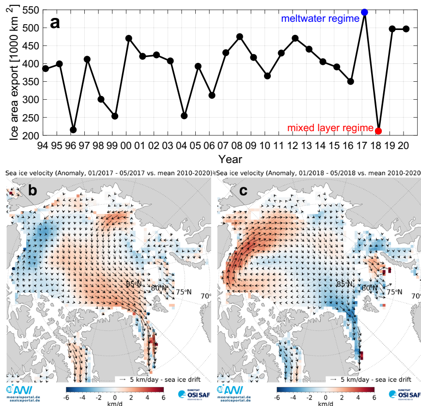
Fig. 2 Fram Strait winter ice export and Arctic winter sea ice velocity anomalies. a Southward sea ice area export [1000 km 2 ] in winter (January to May) between 1994 and 2020 across a zonal gate at 82°N between 12°W and 20°E and a meridional gate at 20°E between 80.5°N and 82°N (see cyan gate in Fig. 1) as used in ref. 105 . The winter values preceding the two discussed stratification regimes are marked. b, c Sea ice velocity [km day -1 ] vectors and anomaly from 2010–2020 mean in color. b is January to May 2017 average and c is January to May 2018 average. Note that the sea ice velocity north of Fram Strait was anomalously large in 2017 and anomalously small in 2018.
