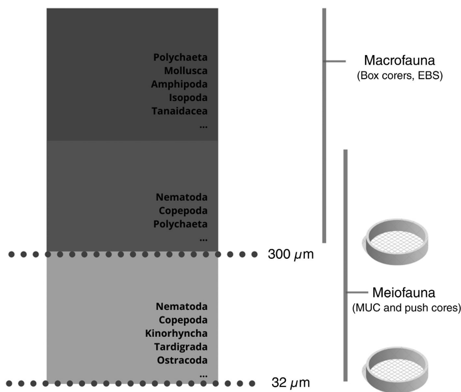
Fig 1. Size limit representations for both meio- and macrofauna based on sieve mesh size and sampling gears. Dark gray colors represent taxa only belonging to the macrofauna, middle gray shows the overlap between meio- and macrofauna groups and light gray exhibit the taxa only belonging to the meiofauna. EBS = epibenthic sledge; MUC = multicorer.
