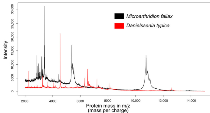
Fig 4. Mass spectra of Microarthridion fallax and Danielssenia typica , two harpacticoid copepod species from the meiofauna of the North Sea. Clear differences between the mass spectra of the two species can be distinguished.
