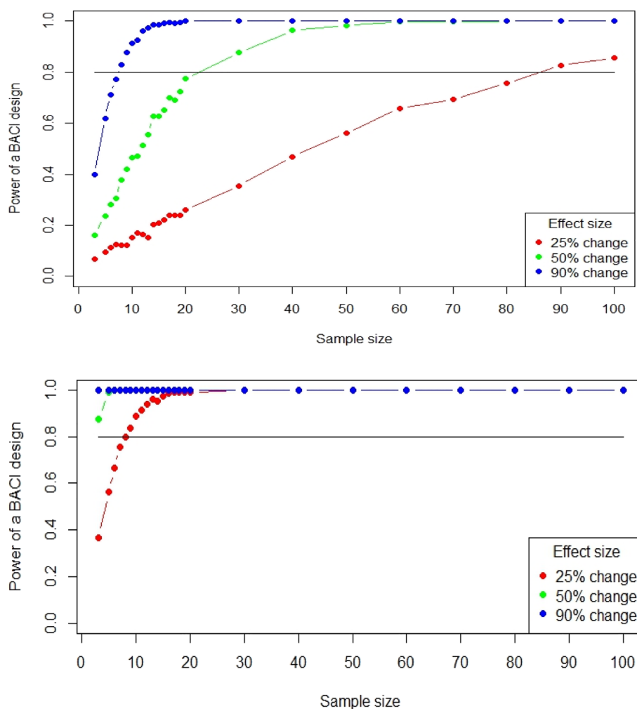
Fig 2. Top—Statistical power of a BACI ANOVA to detect a change in the mean number of macrofauna species, assuming that number of species has a normal distribution of mean = 11.8 and SD = 4.8 as at Domes A, north Equatorial Pacific (Wilson 2017). Bottom—Statistical power of a BACI ANOVA to detect a change in the mean number of nematode genera, assuming that the number of genera has a normal distribution of mean = 47.2 and SD = 5.8 as at the BGR, the German exploration area in the CCFZ (Hauquier et al. 2018).
