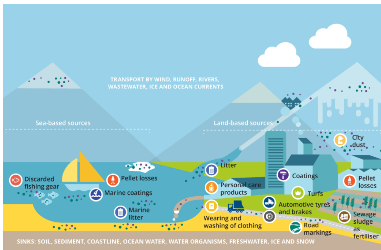
Figure 1. Sources of microplastics, release routes and sinks
