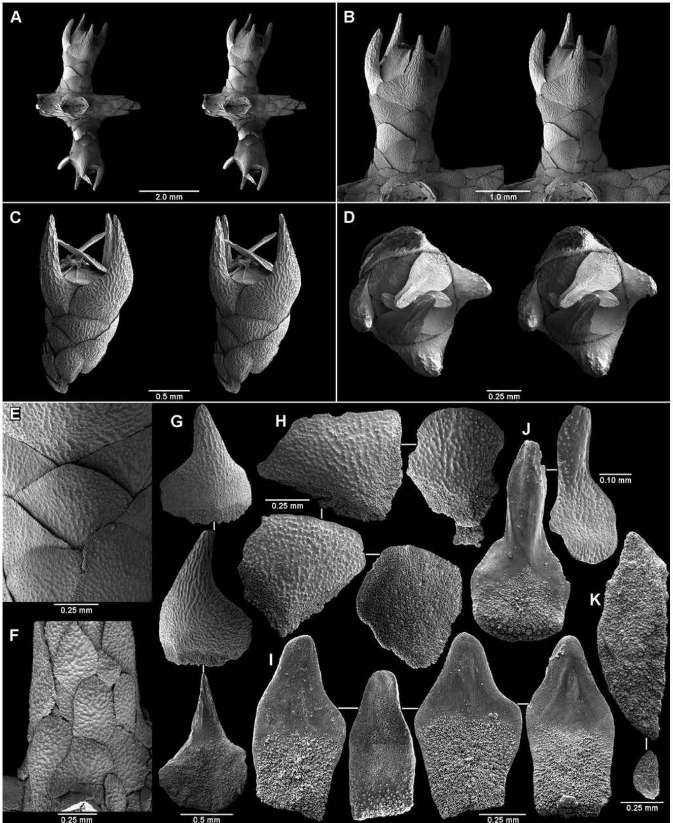
Figure 64. Pachyprimnoa asakoae gen. et sp. nov. , holotype: A. stereo view of a whorl of three polyps; B–C. lateral stereo view of polyps showing massive marginal scales; D. stereo view of operculum surrounded by the four marginal scales; E. marginal scales in situ ; F. coenenchymal scales in situ ; G. massive marginal scales; H. body wall scales; I. upper opercular scales; J. lower opercular scales; K. coenenchymal scales.
