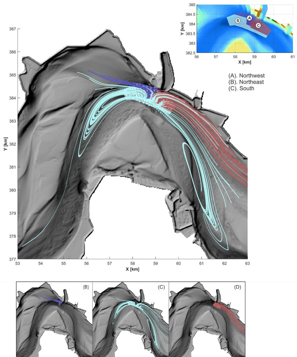
Figure 3.10: Particle trajectories from sources that originate from the Put van Hansweert (grouped in 3 sub-polygons)
