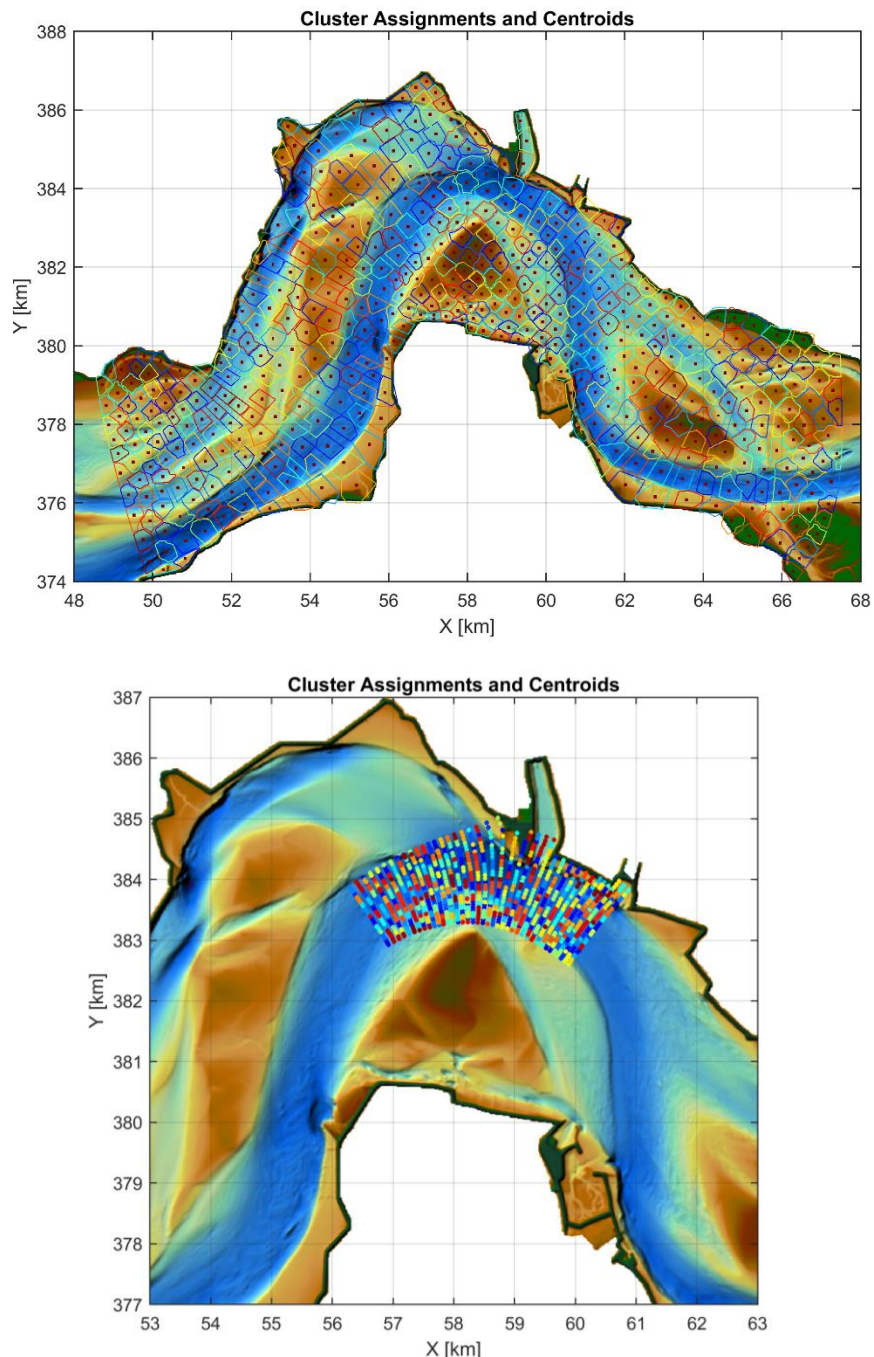
Figure 2.3: Locations of 500 particle sources derived from a cluster analysis on the bathymetric data of the Bocht van Ossenissee (top panel) and the Put van Hansweert (bottom panel).
