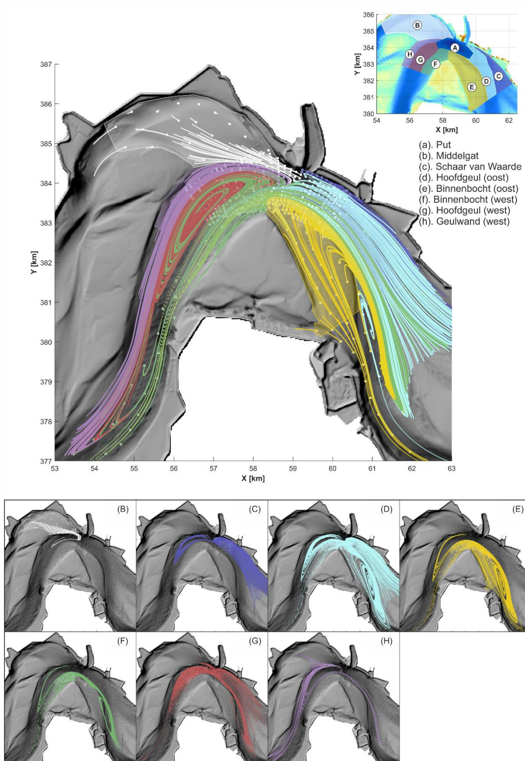
Figure 3.8: Particle trajectories for particles interacting with 7 source locations (individual source particles are grouped by colour) that represent the different morphological elements of the Bocht van Ossensisse (see upper panel). Lower panels; results for the individual areas. Results for sources that interact with Area (A), Put van Hansweert, are visualized in Figure 3.9.
