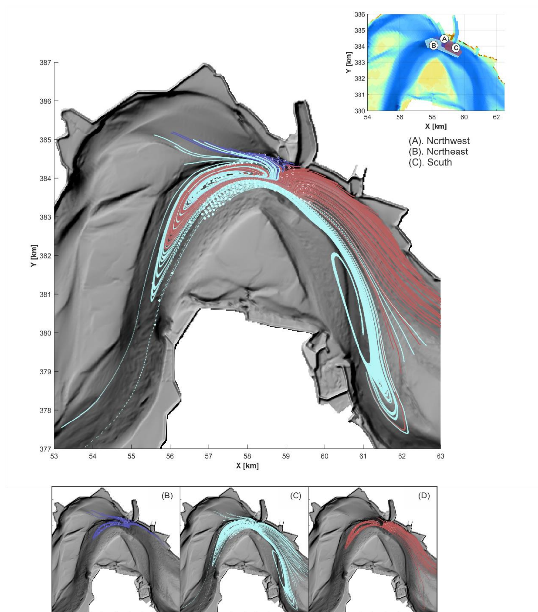
Figure 3.9: Particle trajectories from sources that interact with the Put van Hansweert (grouped in 3 sub-polygons).
