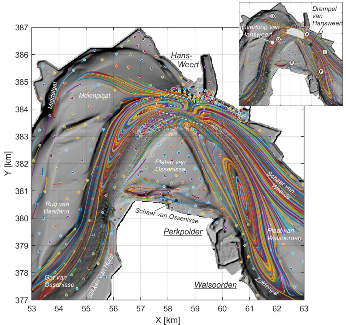
Figure 3.6: Sediment Pathways in the Bocht van Ossenissee. Dots indicate the starting particle source locations and lines illustrate the computed particle trajectories after 1 year of simulation. Colours are used to distinguish the various particle sources.
