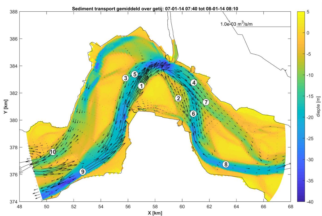
Figure 3.5: Tidally-averaged total sediment transport vectors in the Bocht van Ossenisse.
