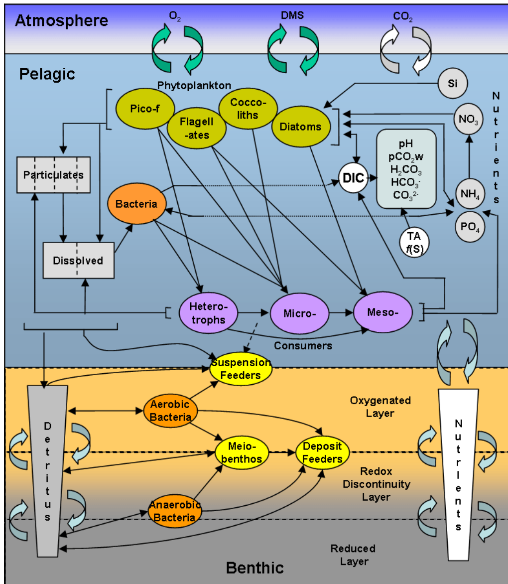
Figure 4.38. ERSEM. Source: MEECE website. http://www.meece.eu/library/ersem.html
