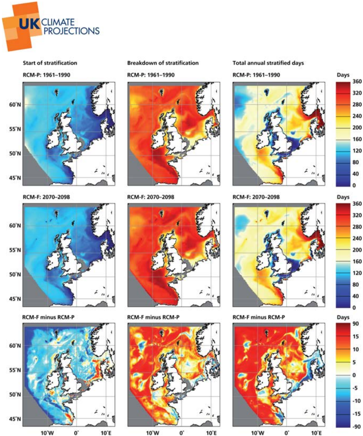
Figure 4.37. Changes in North Sea stratification. Source: Lowe et al. 2009. Figure 6.10
