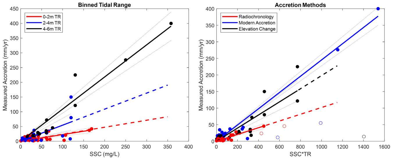
Fig 2. (A) Measured accretion rate is linearly positively related to suspended sediment concentration for a given tidal range (red R^2 = 0.54 , blue R^2 = 0.40 , black R^2 = 0.91 ). (B) Relationship between accretion, SSC, and TR is dependent on methodology, with radiochronology (red, R^2 = 0.80 ) having a significantly lower slope than modern accretion (blue, R^2 = 0.96 ) or elevation change (black, R^2 = 0.72 ). Dashed lines indicate data extrapolation and empty circles indicate the outliers removed from the fit.
