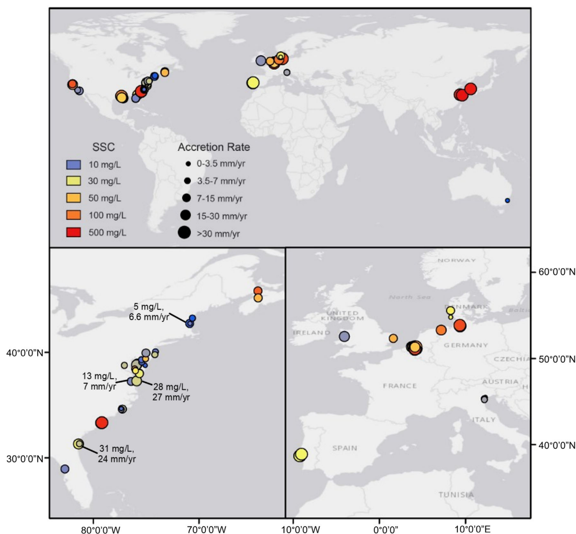
Fig 1. (A) Site map showing SSC and accretion rates of sites used in the meta-analysis. Warmer colors indicate higher SSC and reference values are displayed in the legend. Size of the circle represents accretion rate, with larger circles indicating greater accretion rates. (B) Magnified view of the east coast of North America with labels indicating SSC and accretion rate for the four low marsh monitoring sites and (C) Western Europe.
