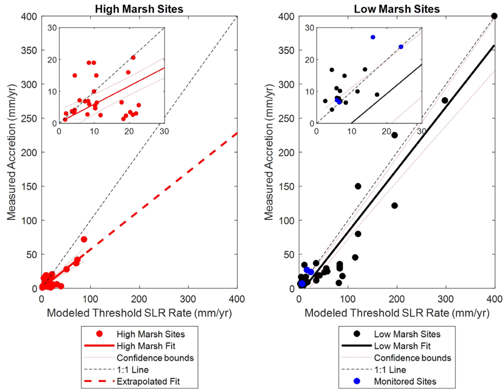
Fig 3. (A) Comparison of observed accretion rate with threshold SLR determined from the ensemble model for high marsh sites ( R^2 = 0.67 , p < 0.01 ). (B) Comparison of observed accretion rate with threshold SLR determined from the ensemble model for only sites that were reported as low marsh ( R^2 = 0.89 , p < 0.01 ). Blue points represent the four low marsh monitoring sites, and the insets are a magnified view of 0–30 \text{mm yr}^{-1} .
