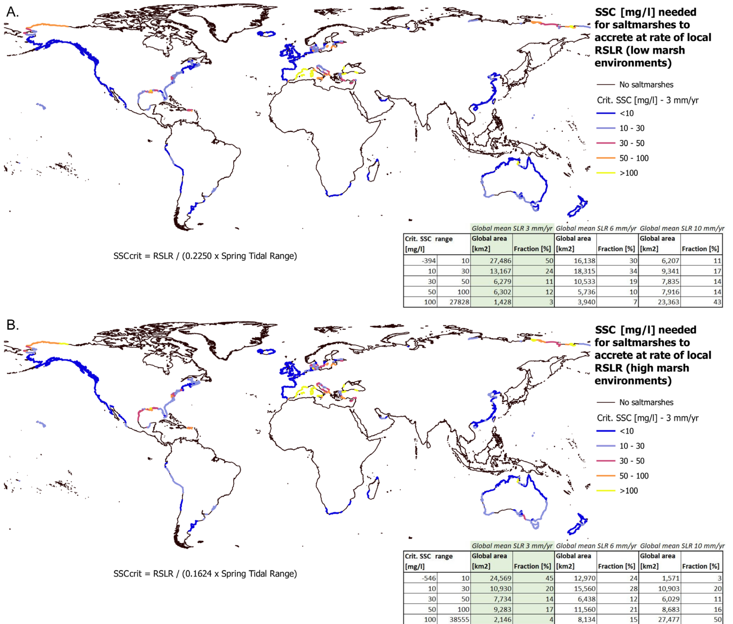
Fig 4. (A) World map indicating critical suspended sediment concentration (SSCcrit) needed for (A) low marshes to survive, or not drown and (B) high marshes to maintain current elevation. Colored segments indicate coastlines where marshes are found.
