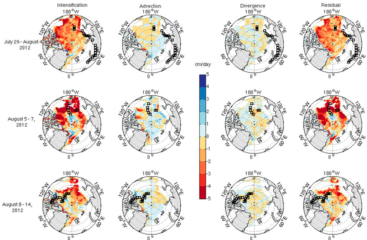
FIG. 7. Sea ice volume budget components including (left to right) intensification, advection, divergence, and residual terms (top) prior to, (middle) during, and (bottom) following the 6 Aug 2012 extreme storm, computed using PIOMAS effective thickness and NSIDC sea ice drift. Units are \text{cm day}^{-1} . Blue (red) values indicate sea ice volume increase (decrease).
