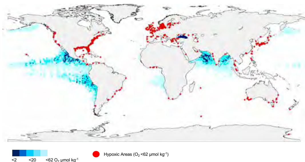
Figure 1.1. Locations of low O 2 areas (i.e. O 2 < 62 μmol kg -1 ) in the coastal and global ocean. In the coastal zone, more than 500 sites have been inventoried with low O 2 conditions in the past half century (red dots); in the open ocean O 2 waters encompass several million km 3 (blue dots refer to conditions at 300 m depth). Source: Adapted from Breitburg et al., 2018.
