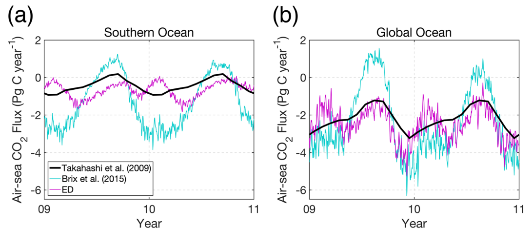
Figure 1. Comparison of daily (a) Southern Ocean and (b) global ocean integrated air-sea CO 2 flux during 2009–2011 from the monthly climatology of Takahashi et al. (2009) (black thick line), Brix et al. (2015) optimized simulation (thin cyan line), and the ED simulation presented in this paper (magenta thin line). The Southern Ocean is defined as all wet grid cells south of 45°S.
