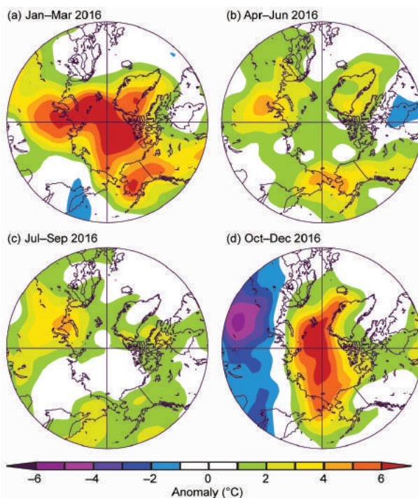
FIG. 5.2. Seasonal anomaly patterns for near-surface air temperatures ( ^{\circ}\text{C} ) in 2016 relative to 1981–2010 in (a) winter (Jan–Mar), (b) spring (Apr–Jun), (c) summer (Jul–Sep), and (d) autumn (Oct–Dec). Temperatures are from slightly above the surface layer (925-mb level) to emphasize large spatial patterns rather than local features. (Source: NOAA/ESRL, www.esrl.noaa.gov/psd/ .)
