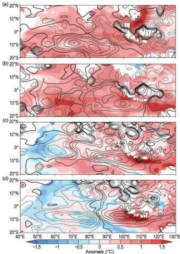
FIG. 4.42. SST ( ^{\circ}\text{C} , colored scale) and precipitation (contour interval: 0, \pm 0.5 , \pm 1 , \pm 2 , \pm 3 , \pm 4 , and \pm 5 \text{mm day}^{-1} ). Solid/dashed lines denote positive/negative values, and thick solid lines indicate zero contour anomalies during (a) Dec 2015–Feb 2016, (b) Mar–May 2016, (c) Jun–Aug 2016, and (d) Sep–Nov 2016. The anomalies were calculated relative to the climatology over the period 1982–2015. [Source: NCEP optimum interpolation SST (Reynolds et al. 2002) and monthly GPCP precipitation analysis ( http://precip.gsfc.nasa.gov ).]
