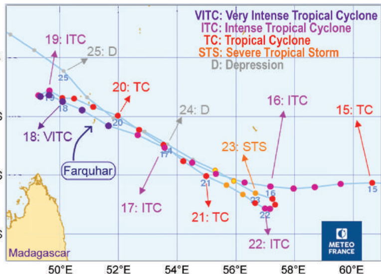
FIG. 7.33. Tropical Cyclone Fantala’s unique trajectory over the Farquhar group (15–25 Apr 2016). (Source: Météo France.)
