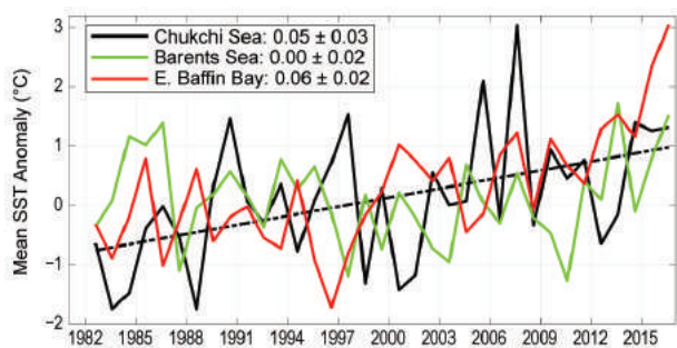
FIG. 5.9. Area-averaged SST anomalies (°C) for Aug of each year relative to the 1982–2010 Aug average for the Chukchi and Barents Seas and eastern Baffin Bay (see Fig. 5.8a). The dashed black line shows the linear SST trend (over the period shown) for the Chukchi Sea. Numbers in the legend correspond to linear trends in °C yr -1 (with 95% confidence intervals).
