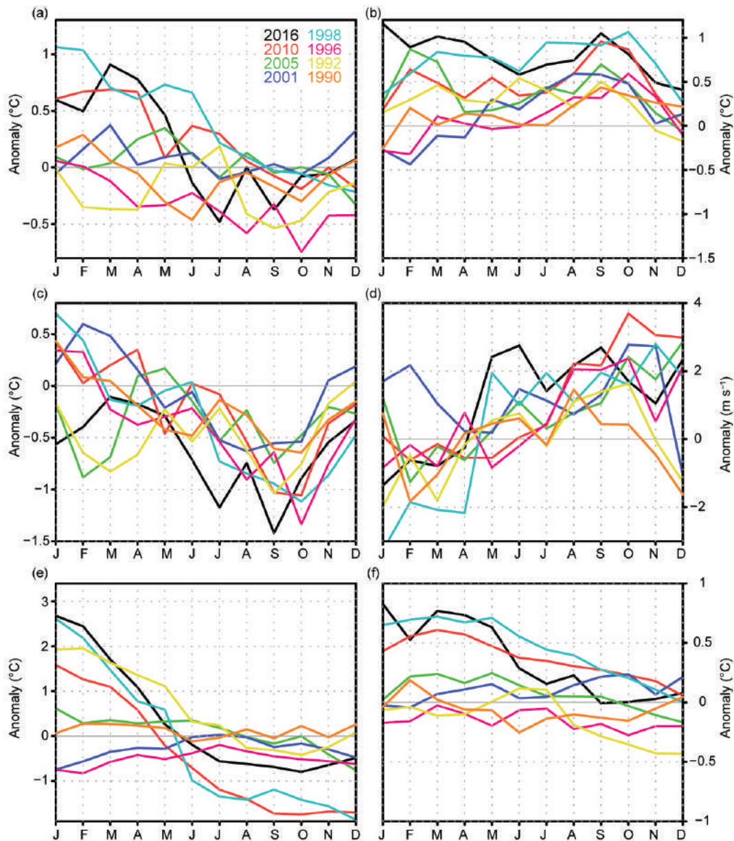
FIG. 4.41. 3-month running mean SST anomalies ( ^{\circ}\text{C} ) in the (a) western IO (IODW; 50^{\circ}\text{--}70^{\circ}\text{E} , 10^{\circ}\text{S--}10^{\circ}\text{N} ), (b) eastern IO (IODE; 90^{\circ}\text{--}110^{\circ}\text{E} , 10^{\circ}\text{S--}0^{\circ} ), and (c) IOD index (measured by the SST anomaly difference between the IODW and the IODE) during eight negative IOD events since 1982. (d) As in (c), but for the surface zonal wind anomaly in the central equatorial IO ( 70^{\circ}\text{--}90^{\circ}\text{E} , 5^{\circ}\text{S--}5^{\circ}\text{N} ). (e),(f) As in (a),(b), but for the monthly SST anomalies in the Niño-3.4 region ( 190^{\circ}\text{--}240^{\circ}\text{E} , 5^{\circ}\text{S--}5^{\circ}\text{N} ) and the tropical IO basin ( 40^{\circ}\text{--}120^{\circ}\text{E} , 20^{\circ}\text{S--}20^{\circ}\text{N} ). The monthly anomalies were calculated relative to the climatology over the period 1982–2015. These are based on the NCEP optimum interpolation SST (Reynolds et al. 2002) and JRA-55 atmospheric reanalysis (Ebita et al. 2011).
