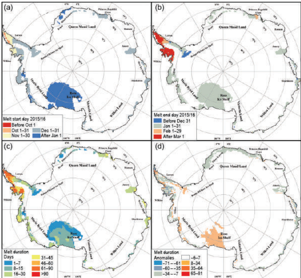
FIG. 6.6. Estimated surface melt for the 2015/16 austral summer: (a) melt start day, (b) melt end day, (c) melt duration (in days), and (d) melt duration anomalies (in days).
