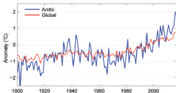
FIG. 5.1. Arctic and global average annual land surface air temperature (SAT) anomalies ( ^{\circ}\text{C} ) for 1900–2016 relative to the 1981–2010 average. Note that there were few stations in the Arctic, particularly in northern Canada, before 1940. (Source: CRUTEM4 dataset, www.cru.uea.ac.uk/cru/data/temperature .)
