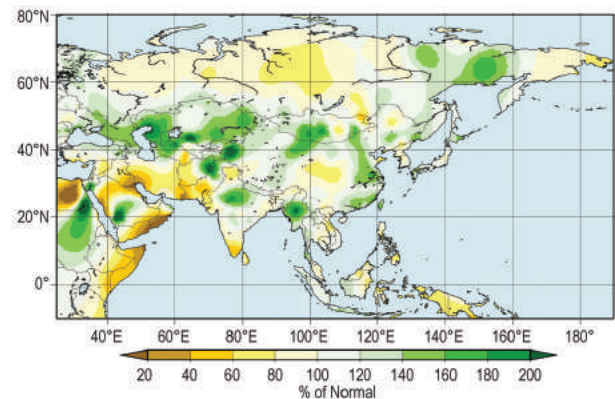
FIG. 7.41. Annual precipitation (% of normal; 1981–2010 base period) over Asia in 2016. (Source: Japan Meteorological Agency.)
