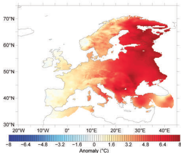
Fig. 7.39. Monthly mean air temperature anomalies for Feb 2016 (°C; 1961–90 base period), based on E-OBS data (van der Schrier et al. 2013b; Chrysanthou et al. 2014). (Source: KNMI.)
