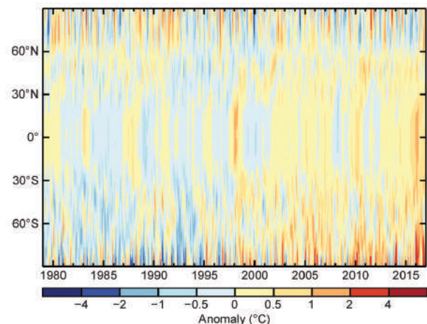
FIG. 2.7. Latitude–time cross-section of lower tropospheric temperature anomalies (°C) relative to 1981–2010 from ERA-Interim (Dee et al. 2011).
