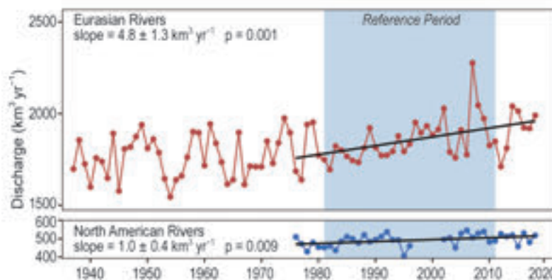
FIG. 5.24. Long-term trends in annual discharge ( \text{km}^3 \text{yr}^{-1} ) for Eurasian and North American Arctic rivers. Gaps in the North American rivers time-series span from 1996 to 2001 due to missing Yukon data from 1996 to 2001 and missing Mackenzie measurements in 1997 and 1998. Note the different scales for the Eurasian and North American river discharge; discharge from the former is 3–4 times greater than from the latter.
