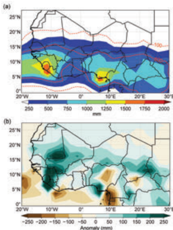
FIG. 7.22. Jun–Sep 2018 precipitation for West Africa as (a) total accumulated precipitation (mm) and (b) anomalies (mm; base period: 1981–2010). The red dashed and solid lines in (a) mark 100 mm and 600 mm isohyets. (Source: NOAA/NCEP.)
