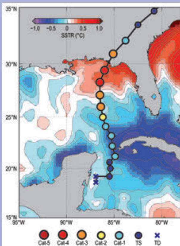
FIG. SB4.4. SSTR residuals (seasonal cycle removed), showing the difference between mean SSTs during Sep 2018 and the historical mean SSTs for Sep during 1985–2018.
