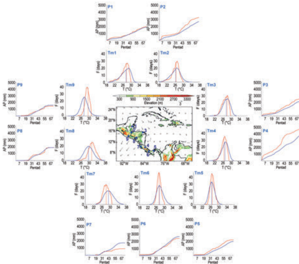
FIG. 7.8. Mean surface temperature (Tm; °C) frequency (F; days), and accumulated pentad precipitation (P; mm) time series are shown for nine stations in Central America: (1) Philip Goldson International Airport, Belize; (2) Puerto Barrios, Guatemala; (3) Puerto Lempira, Honduras; (4) Puerto Limón, Costa Rica; (5) Tocumen International Airport, Panamá; (6) David, Panamá; (7) Liberia, Costa Rica; (8) Choluteca, Honduras; and (9) Puerto San José, Guatemala. The blue solid line represents the 1981–2010 average values and the red solid line shows 2018 values. Vertical dashed lines show the mean temperature for 2018 (red) and the 1981–2010 period (blue). Vectors indicate Jul wind anomalies at 925 hPa (1981–2010 base period). Shading depicts regional elevation (m). (Sources: NOAA/NCEI and CA-NWS.)
