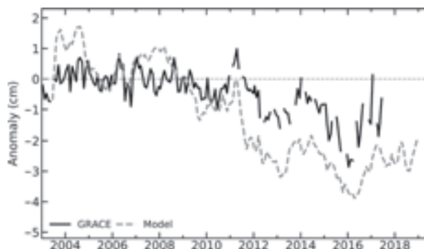
FIG. 2.28. Global average terrestrial water storage anomalies from GRACE (black) and from a GRACE data assimilating land surface model (gray), in cm equivalent height of water relative to a 2005–10 mean baseline.
