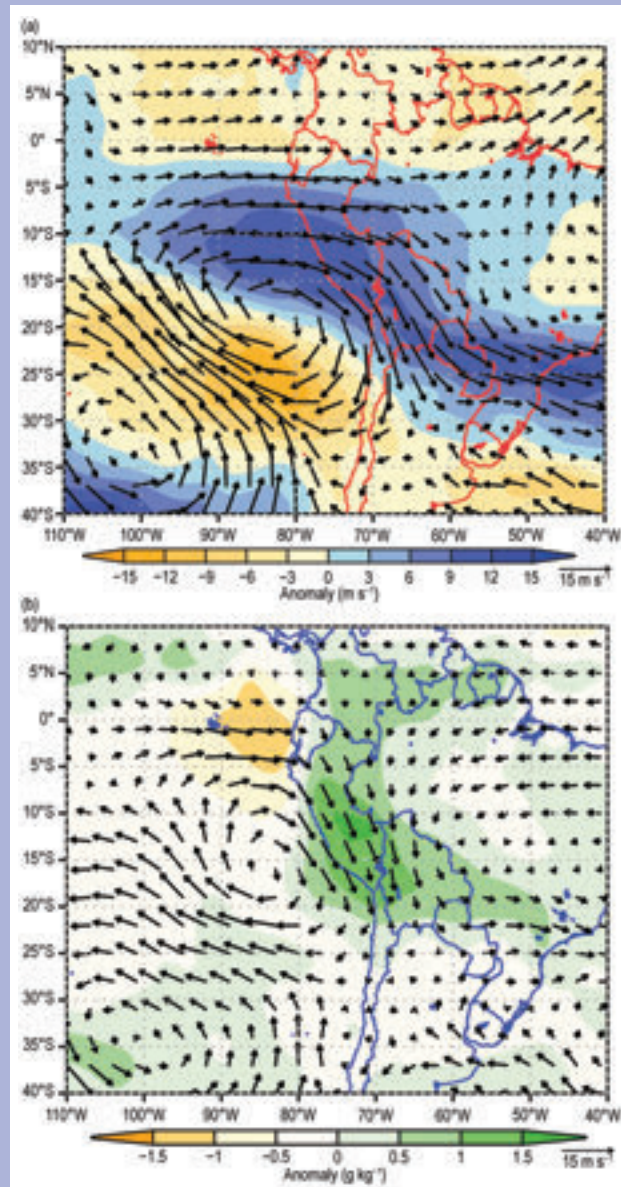
Fig. SB7.5. Composite anomaly map of (a) 250-hPa wind (vectors) and magnitude (shaded, m s^{-1} ), and (b) 500-hPa wind (vectors) and humidity mixing ratio (shading; g kg^{-1} ), of seven extreme snowfall events occurred Jun–Aug 2018. (Source: ERA-interim.)
