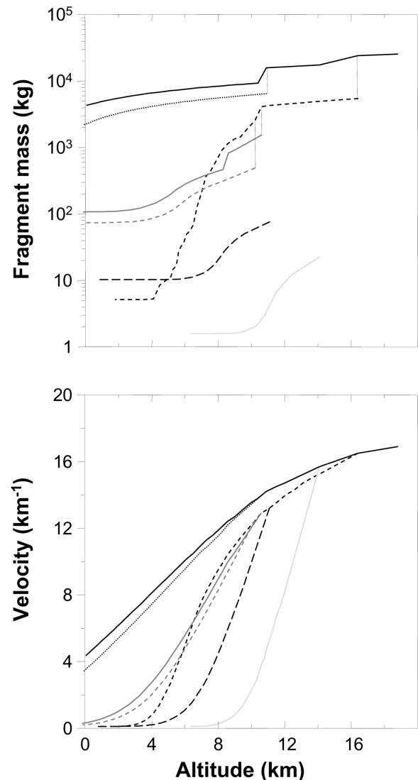
Fig. 10. The mass (top) and velocity (bottom) of iron fragments disrupted in the atmosphere. This figure traces the evolution of a given fragment down into the atmosphere. Different fragments are represented by different shades or dashes. The first disruption occurs at an altitude of 16 km. Smooth decreases in mass are due to ablation; sharp ones (vertical lines in the upper plate) are due to fragmentation.
