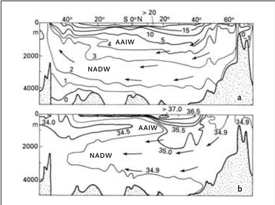
Figure 2 North-south section in the western Atlantic Ocean showing the temperature (a) and the salinity (b) as a function of depth.
