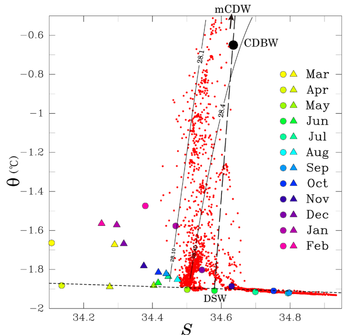
Fig. 4. Potential temperature-salinity ( \theta - S ) diagram for mooring data. The monthly mean water properties are represented as circles for a1 and triangles for the upper layer at a2, color-coded by month. Red dots represent the lower layer at a2 at 6-hour intervals from August 20 to September 10. The mean \theta and S of the CDBW outflow obtained from Ohshima et al. (7) is denoted by the solid black circle. The mixing line of CDBW connecting mCDW to pure (freezing point) DSW is shown as a dashed line. The freezing temperature line is shown as a dotted line. Isolines of neutral density ( \text{kg m}^{-3} ) are given as thin black curves.
