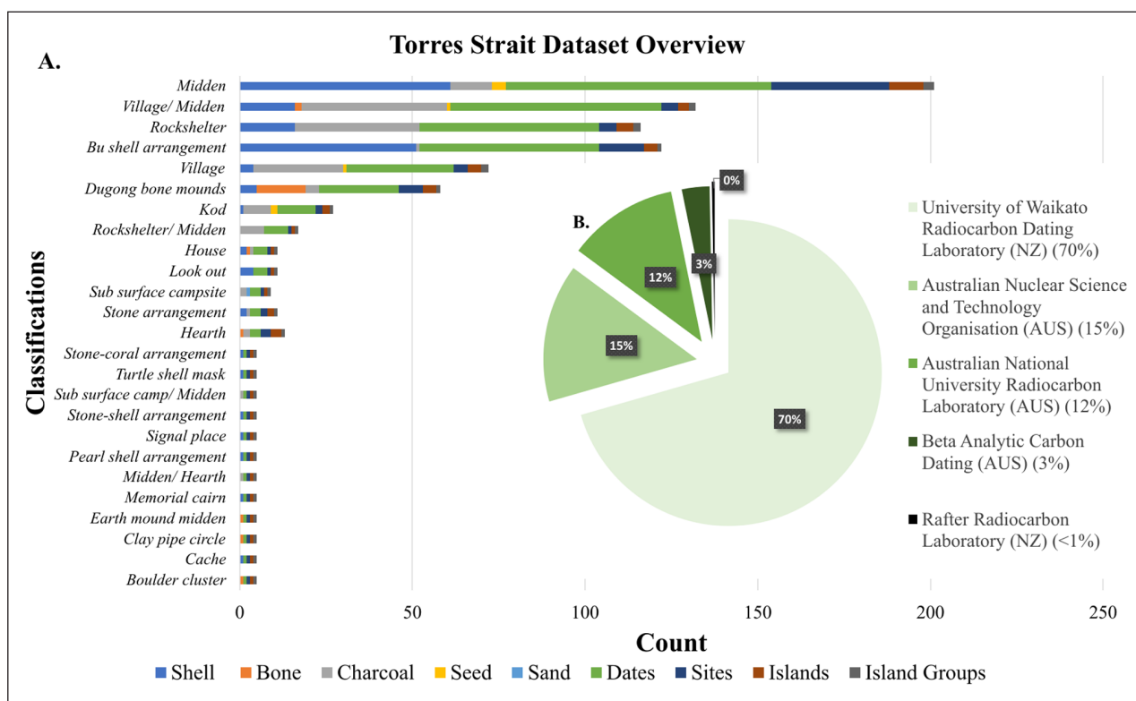
Figure 2 (A) Breakdown by sample and site classification of 14 C ages in the Torres Strait Radiocarbon Database: version 2.0 [7], including (B) the percentage of ages dated from different radiocarbon dating laboratories.
