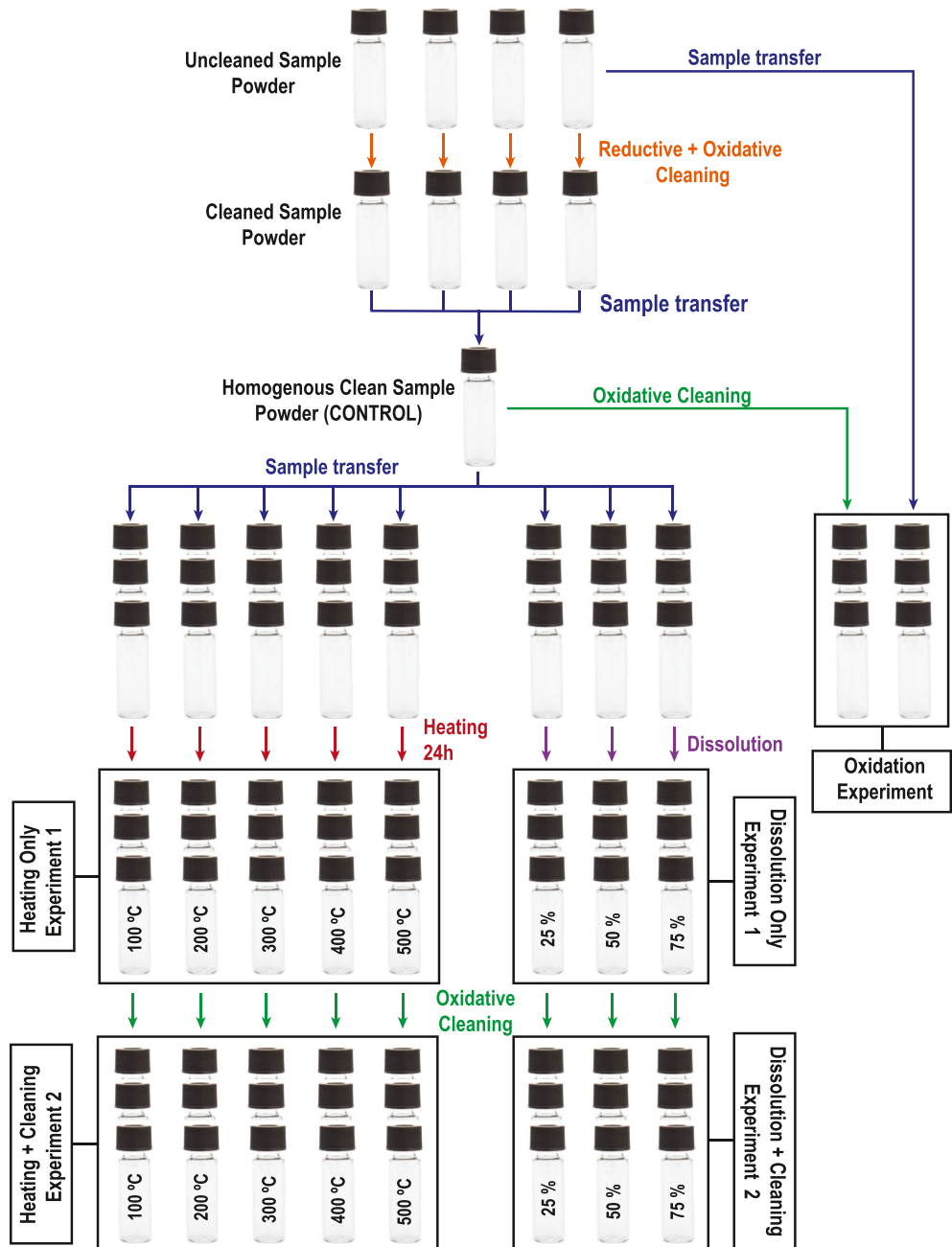
Figure 1. Experimental Design. For each sample type, an aliquot of uncleaned powder was taken and used in our chemical oxidation experiment. The remaining powder was subsequently cleaned in four aliquots (of 50 mg each) following the reductive-oxidative cleaning methods described in Section 2.3. After the cleaning, the dry fossil powder was combined in a single vial and homogenized. This homogenous, cleaned powder was measured (at least in triplicate) and used as a control sample for all of our treatments. In our oxidation experiment, the uncleaned sample aliquot was measured in triplicate and compared to our (cleaned) control sample, and to an aliquot of the control sample that was divided in triplicate, oxidatively cleaned for a second time, and measured. In our dissolution experiments, we performed three triplicate treatments in which approximately 25%, 50%, and 75% of the control sample was dissolved. In our first dissolution experiment, the sample powders remaining after dissolution were rinsed five times with Milli-Q water and measured. In our second experiment, the powders were recleaned oxidatively before measurement. In our heating experiments, the control sample powder was heated to 100°C, 200°, 300°, 400°, and 500°C. In our first experiment, samples were measured directly after heating; in our second experiment, samples were recleaned oxidatively before the measurement.
