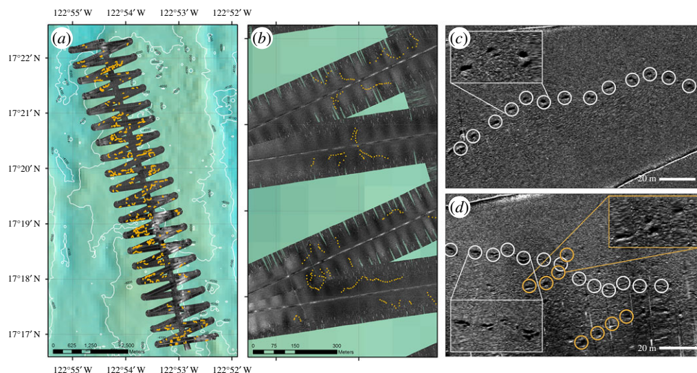
Figure 3. Autosub6000 Mission 81 (M81) within APEI. (a) High-frequency (410 kHz) side-scan sonar acquired at 3 m altitude. Areas with high acoustic backscatter are represented in light grey, low acoustic backscatter in dark grey. Orange circles indicate depressions that have been digitized in ArcGIS 10.3. (b) Zoom of M81 indicating sequential depressions or 'tracks'. (c) Single sequence of depressions (track) from M81. Depth: 4023 m. (d) Overlapping tracks of differing ages. White tracks show high contrast and sharp edges indicating relatively younger tracks than those in orange with lower contrast and less definitive edges. Depth: 4041 m.
