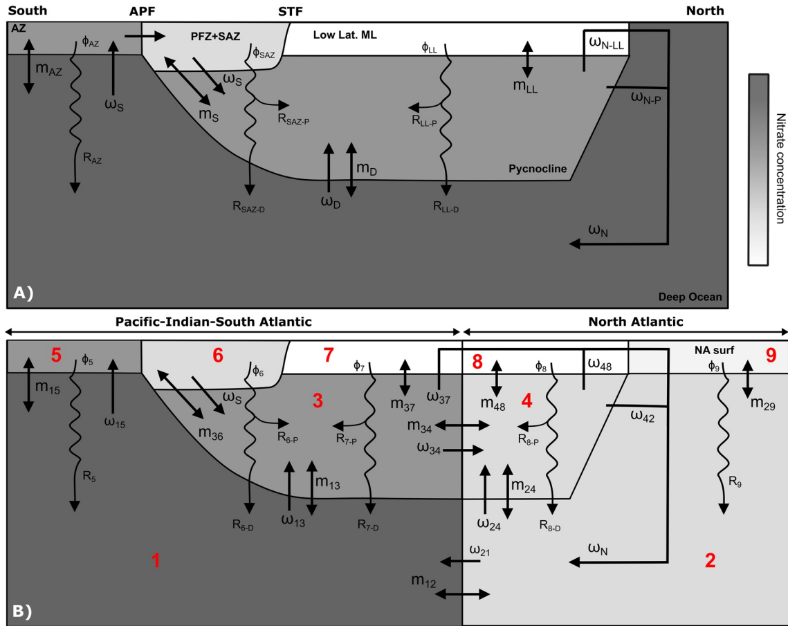
Figure 3. Schematics of the reservoirs and processes included in the prognostic five-box ocean model (a; adapted from Fripiat, Martínez-García, et al., 2021) and in the prognostic nine-box ocean model (b). Straight arrows represent water exchange fluxes either by large-scale advection ( \omega terms) or mixing ( m terms), while wavy arrows indicate export production and remineralization. These terms are described in Table 1. The addition and removal of nitrate by N_2 fixation and denitrification are not shown and are confined to the pycnocline and the overlying surface (see Section 3.1.2). In Text S2 in Supporting Information S1, a model version is described that includes a portion of N_2 fixation and sedimentary denitrification occurring in the deep ocean. Abbreviations are as follows: AZ, Antarctic Zone; PFZ, Polar Front Zone; SAZ, Subantarctic Zone; APF, Antarctic Polar Front; STF, Subtropical Front; Low Lat. ML, low latitude-mixed layer; NA surf, North Atlantic surface water.
