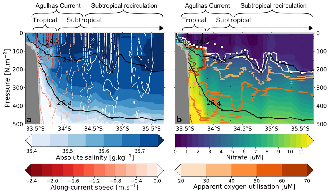
Figure 2. Structure of the Agulhas Current and recirculating waters. (a) Gridded depth section of absolute salinity [g.kg -1 ] over the upper 500 m of the ASCA16 transect. Overlaid in shades of red are contours of along-current speed [m.s -1 ] measured from a shipboard acoustic Doppler current profiler. (b) Gridded depth section of nitrate concentration [μM] over the upper 500 m of the ASCA16 transect. Overlaid in shades of orange are contours of apparent oxygen utilization (AOU) [μM]. Small white circles indicate the mixed layer depth at each station. In both (a and b), black contours show the isopycnal boundaries of the major water masses (see Table 1). The top row of brackets indicates the position of the fast-flowing Agulhas Current and adjacent subtropical recirculation. The bottom row of brackets distinguishes the fresh, high-AOU, high-nitrate, tropically sourced waters along the inshore side of the Agulhas Current from the saline, lower-AOU, lower-nitrate, subtropically sourced waters along the offshore side of the Agulhas Current. The shoaling isopycnals that uplift nutrient-rich waters within the Agulhas Current are consistent with observations of subsurface nutrient streams reported in other WBCs (Pelegrí & Csanady, 1991).
