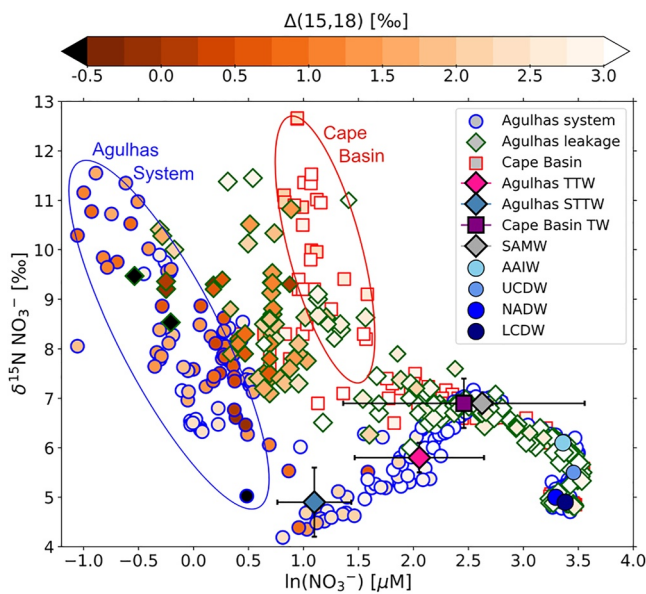
Figure 8. Tracking Agulhas leakage into the South Atlantic Ocean. Data from ASC16 and the subtropical South Atlantic plotted in nitrate \delta^{15}\text{N} [‰] versus \ln([\text{NO}_3^-]) [ \mu\text{M} ] space (i.e., “Rayleigh space”), with symbol color indicating nitrate \Delta(15-18) [‰]. Symbol shape and outline-color indicate the sampling region, except for the bold diamond markers outlined in black, which show the mean \ln([\text{NO}_3^-]) and concentration-weighted nitrate \delta^{15}\text{N} measured for Subantarctic Mode Water (SAMW; gray), Agulhas Subtropical Thermocline Water (STTW; blue), and Agulhas Tropical Thermocline Water (TTW; pink), as well as the purple square, which shows Cape Basin Thermocline Water (TW). In addition, the mean \ln([\text{NO}_3^-]) and concentration-weighted nitrate \delta^{15}\text{N} are shown for Antarctic Intermediate Water (AAIW), Upper Circumpolar Deep Water (UCDW), North Atlantic Deep Water (NADW), and Lower Circumpolar Deep Water (LCDW), as measured in the Agulhas region. Four data sets that sampled both “background” Cape Basin conditions (squares outlined in red) and Agulhas leakage (diamonds outlined in green) are included on the plot: VOY016 cruise (Smart et al., 2020), SAMBA: South Atlantic MOC Basin-wide Array 2015 (Marconi et al., 2017) and 2017 (R. Granger et al., 2023), and VOY03 cruise (Smart et al., 2015).
