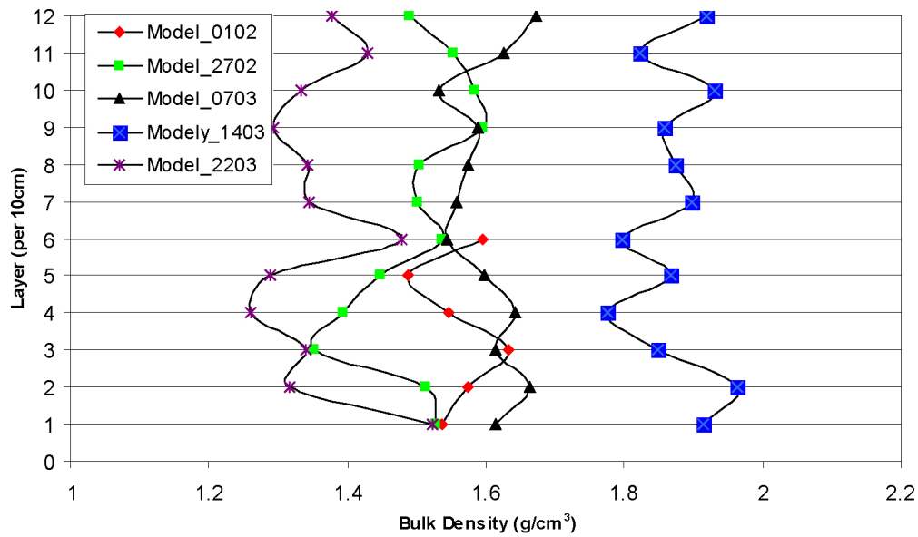
Figure 27 Model Material Dry Density Distributions
