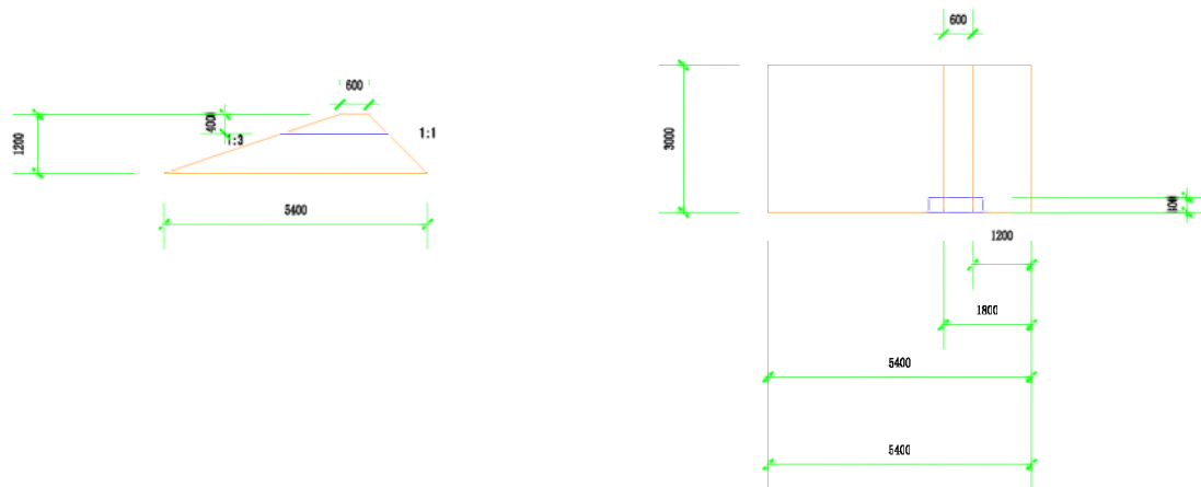
Figure 12 Design of Model 4
