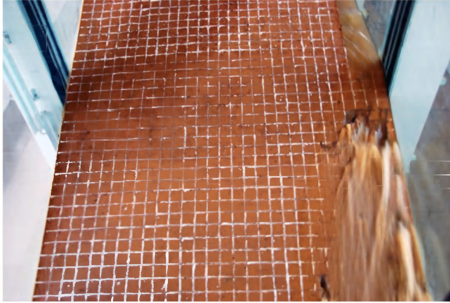
Figure 38 Surface Erosion at the initial phrase of breach
