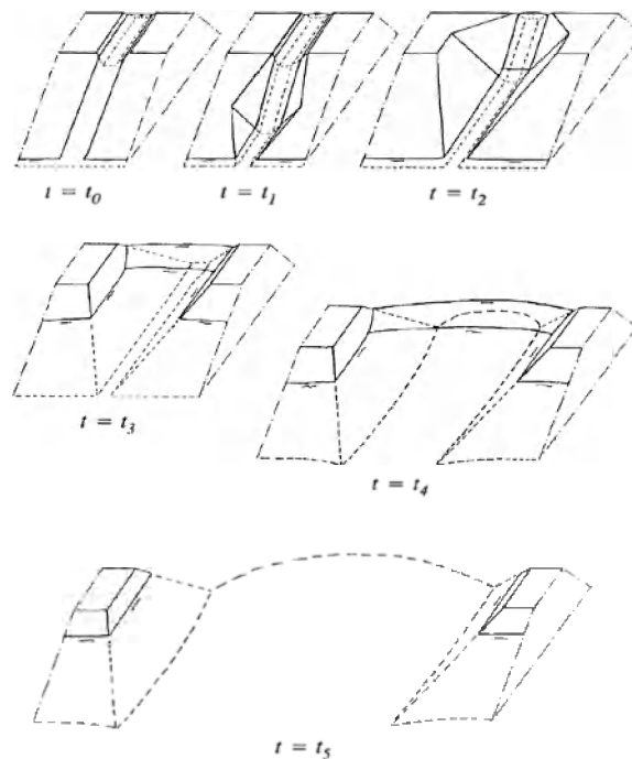
Figure 1 Schematic illustration of breach growth in a sand-dike (Visser, 1998)
