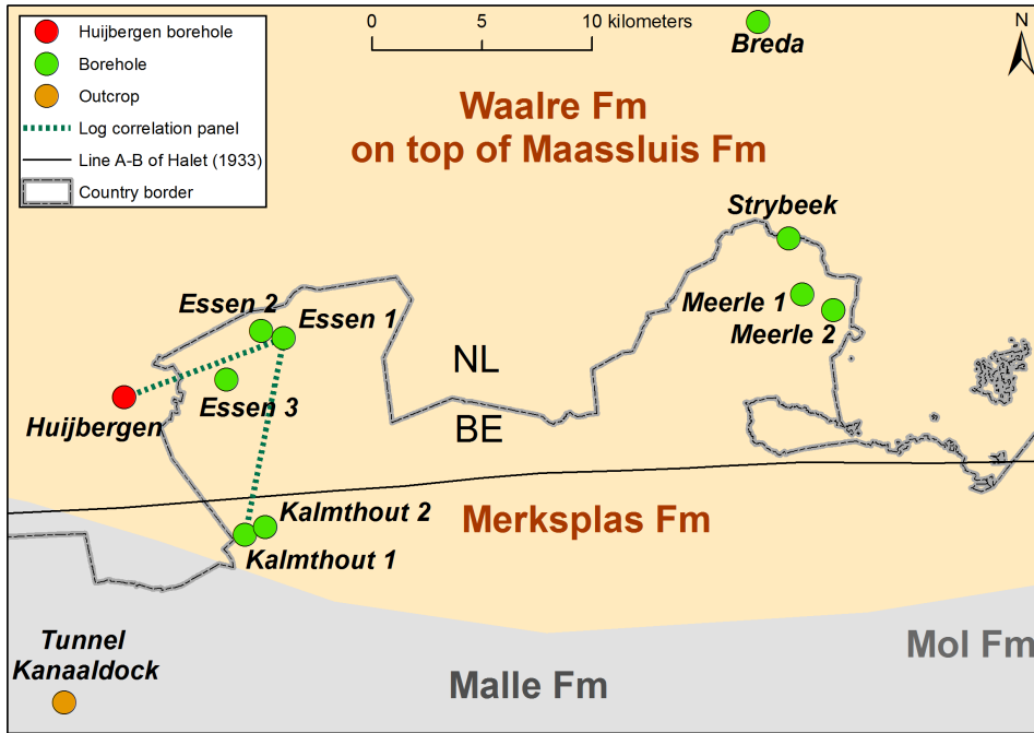
Figure 1. Location of the study area near the Dutch/Belgian border with the geographic extent of the main stratigraphic units and the relevant boreholes/outcrops (Table 1). The correlation panel of Fig. 4 is also indicated.
