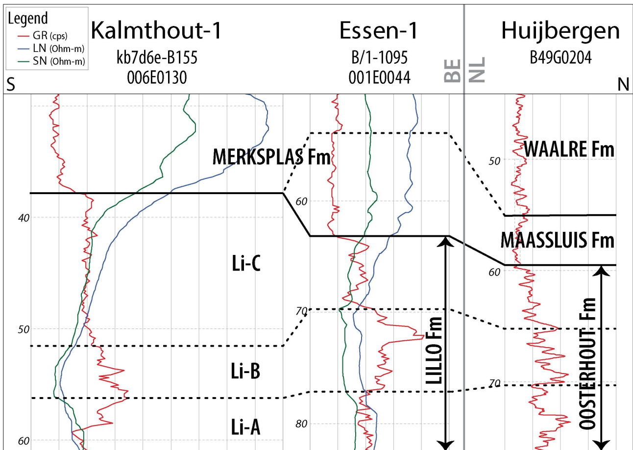
Figure 4. Borehole-log correlation panel for the Pliocene and Lower Pleistocene stratigraphic units along a N–S transect from northernmost Belgium across the border with the Netherlands (location of the profile: see Fig. 1). The original correlation panel of Louwye et al. (2020) is modified by this study. GR: gamma-ray. LN: long-normal (resistivity). SN: short-normal (resistivity).
