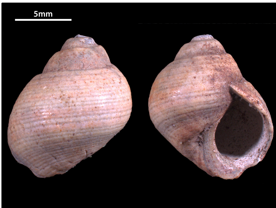
Figure 5. RGM.1365361. Littorina littorea Linnaeus, 1758 from sample 58–59 m, Maassluis Formation, borehole Huijbergen.
