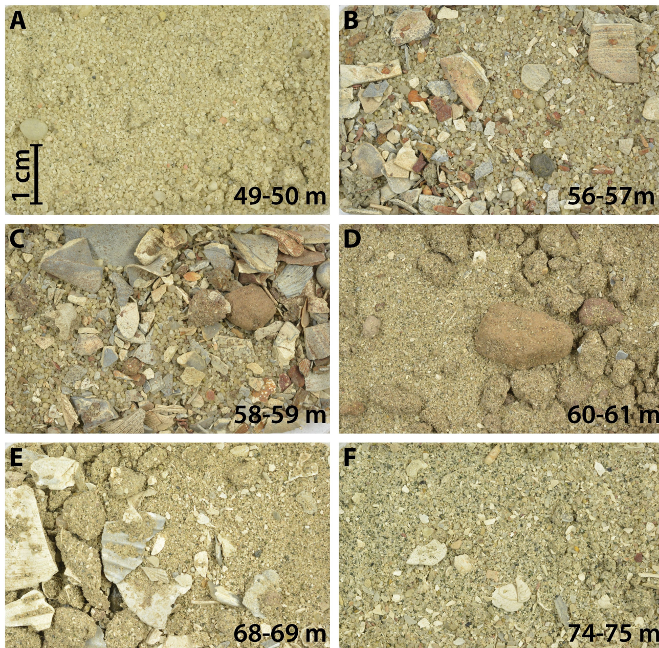
Figure 3. Sediment samples of the Huijbergen borehole. (A) Sample 49–50 m (RGM.1365353) contains quartz grains and lacks calcareous fossils. It represents the Waalre Formation. (B) Samples 56–57 (RGM.1365354) and (C) 58–59 m (RGM.1365355) contain poorly sorted, mostly coarse-grained quartz sand with abundant, mostly abraded, shell fragments. Some clast pebbles and gravel are found. This interval is attributed to the Maassluis Formation. (D) Sample 60–61 m (RGM.1365356) contains slightly oxidised quartz grains, (very) little glauconite, fine shell fragments and lithified brown-red clay nodules with small shell fragments. The sample is attributed to the Oosterhout Formation. (E) Samples 68–69 m (RGM.1365357) and (F) 74–75 m (RGM.1365358) are characterised by poorly sorted, fine-grained quartz sand rich in shells and shell fragments attributed to the Oosterhout Formation. Sediments in the Maassluis Formation samples are notably coarser grained than in the Oosterhout Formation samples, while they lack glauconite.
