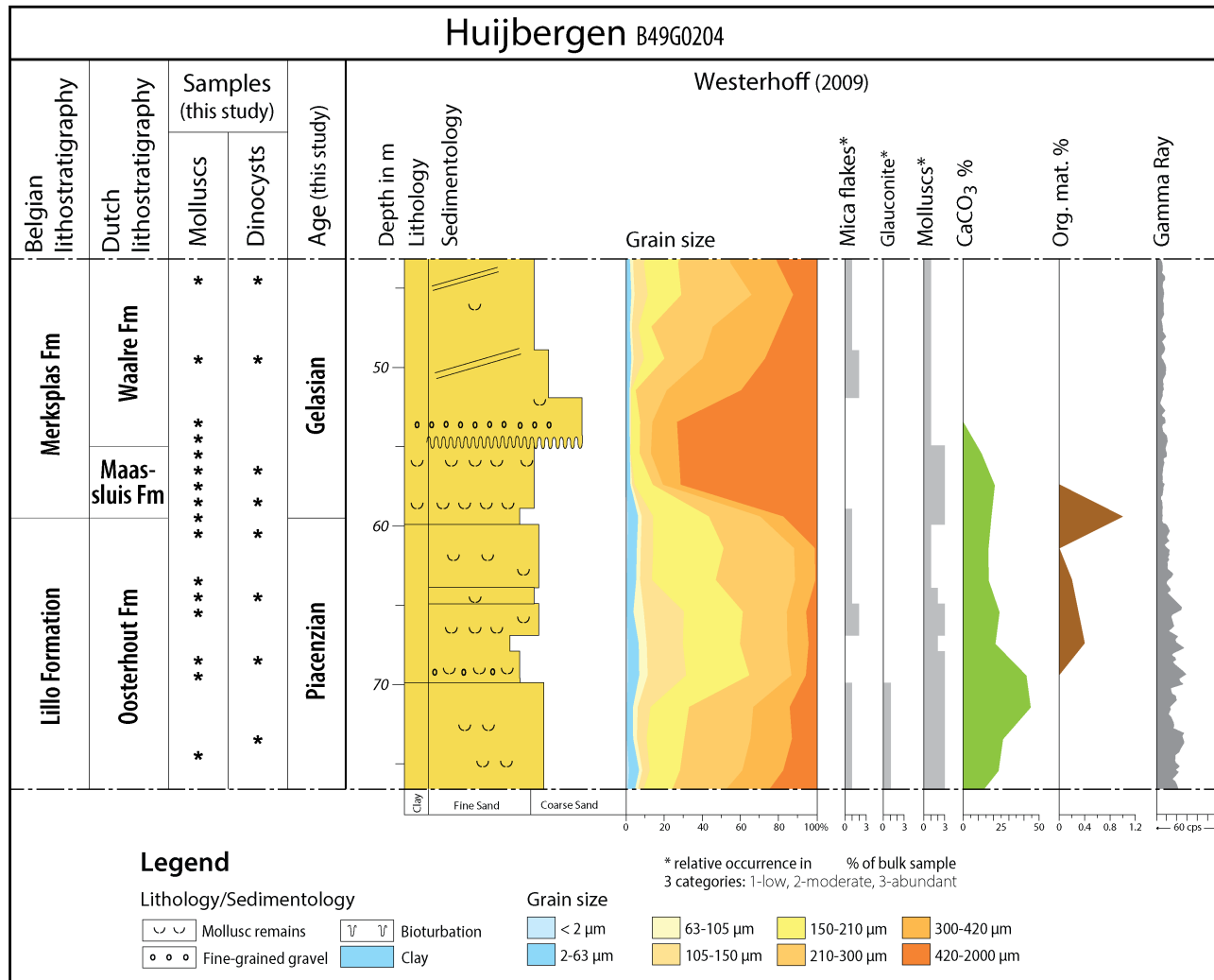
Figure 2. Borehole Huijbergen with lithostratigraphic interpretation (see 4.1.), dinocyst and mollusc sample locations and age assessments on the left side (this study). In the center and on the right side, a sketch of the original lithological description, results of grain-size analyses and data on mica flakes, glauconite content, relative abundance of molluscs, CaCO 3 %, organic matter (%) and a gamma-ray log (data from Westerhoff, 2009).
