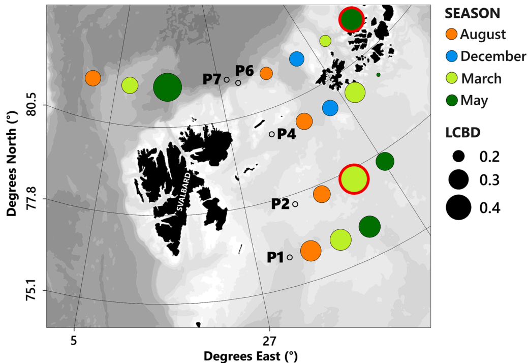
Fig. 7. Map showing the results of the Local contribution to beta diversity (LCBD) for the Hellinger transformed macrofauna abundance in the northern Barents Sea across four seasons. The position of each station is indicated with empty circles. LCBD values for each station across seasons are indicated with colored circles the sizes of which indicate the LCBD value and the color the season. LCBD values are calculated individually for each station comparing seasons and therefore should not be compared between locations. LCBD indices from seasons which are significant are indicated with a red rim ( p adjusted-value < 0.05 after applying the Holm correction for multiple testing) indicating seasons that are more unique in community composition than the average composition of the other seasons.
