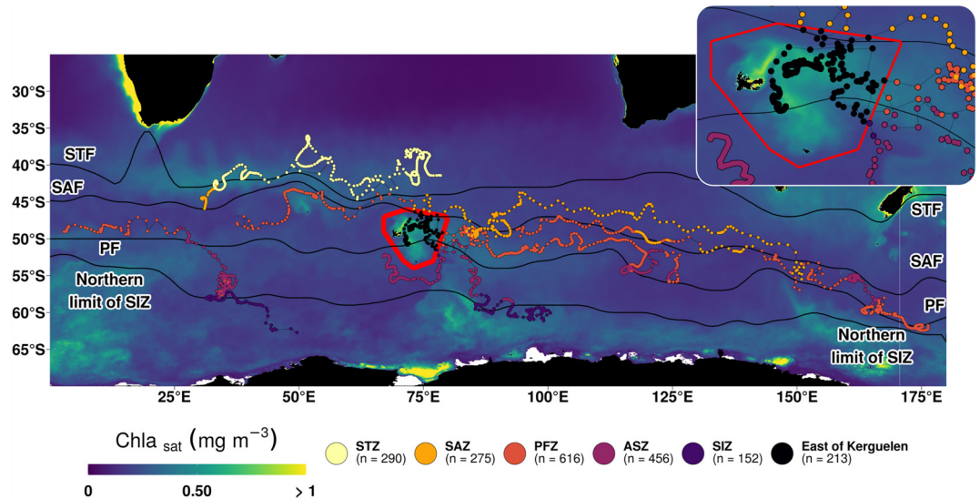
Figure 1. Sampling of the Southern Ocean by the seven floats equipped with transmissometers. Dots indicate the position of profiles. Dot colors refer to the various biophysical zones, delineated by the position of fronts and the extent of September sea-ice coverage (black lines). Fronts were located with Gray et al. (2018)'s criteria applied on climatologies of temperature (product accessible here https://doi.org/10.48670/moi-00052 and based on Guinehut et al. (2012); Mulet et al. (2012)). The boundaries of the zone called “East of Kerguelen” are drawn in red and detailed in the top right insert. The background map is the Spring-Summer climatology (2015–2019) of satellite [Chl- a ] (product accessible here https://doi.org/10.48670/moi-00280 and based on Antoine and Morel (1996); Gohin et al. (2002); Hu et al. (2012); O’Reilly et al. (1998, 2000).
