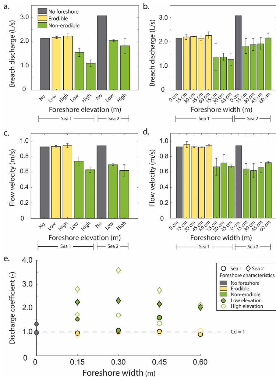
Fig. 5. The effect of foreshore characteristics on breach hydrology. Averaged breach discharge (Q) (a,b) and flow velocity (u) (c,d), presented per group of foreshore characteristics for settings Sea 1 and Sea 2. Note that Q for Sea 2 are higher due to a larger sea area inside the flume. Results are grouped by foreshore elevation (a,c) and by foreshore width (b,d). Error bars indicate standard deviation. (e) Discharge coefficient (Cd) for each run. Cd = 1 shows no additional foreshore effect. Values in Supplementary material.
