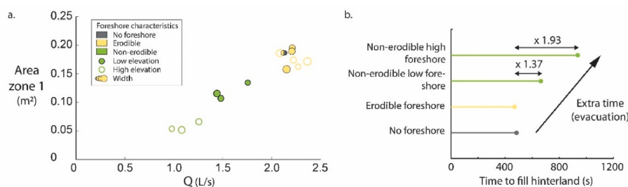
Fig. 6. Flood impact in the mimicked hinterland. (a) Size of the proxy for the breach zone (Area zone 1 in m 2 ) plotted against breach discharge (Q in L/s) for run 01–15. Different foreshore widths indicated by dot size. (b) Hinterland filling time (time to fill first overflow tank-set), based on the constant breach discharge as calculated for the linear phase in each run. Averaged values per group for run 01–15. Values in Supplementary material.
