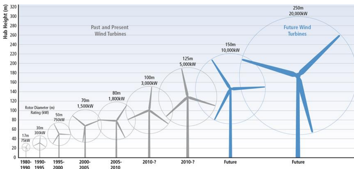
Box 1-3 Design trends: turbine rotor diameter
