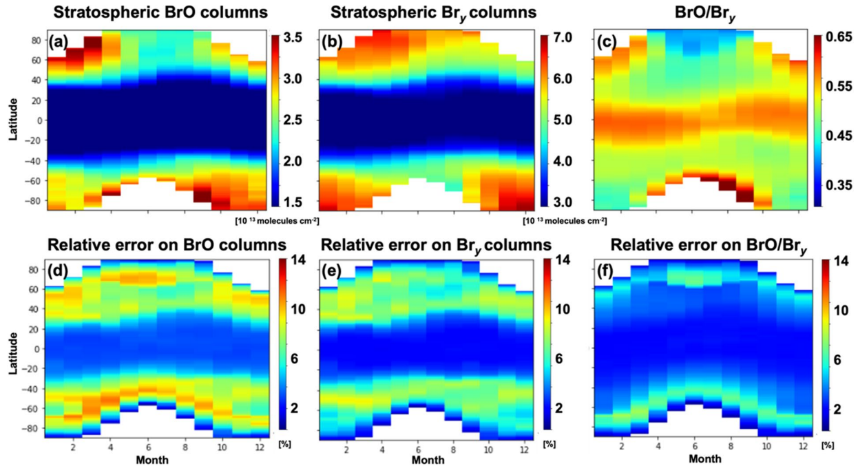
Figure 2. Monthly and zonal averaged stratospheric BrO columns from the GEOS-Chem high performance (GCHP) simulations (a) along with the associated dynamical (stratospheric \text{Br}_y columns; b) and chemical (BrO/ \text{Br}_y ) parameterization (c). Relative error (defined by the ratio of standard deviation to mean) for stratospheric BrO columns (d), dynamical indicator (e), and chemical indicators (f) are also shown.
