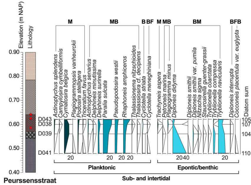
Fig. 8. Percentage diatom diagram reconstructing the aquatic palaeoenvironment at Peursensstraat (exaggeration \times 10 , lithology key Fig. 5, selected taxa). M = marine; B = brackish; F = freshwater. The taxonomy follows Witkowski et al. (2000), Krammer & Lange-Bertalot (2008) and Bey & Ector (2013). The current accepted names were verified according to Algaebase (Guiry & Guiry 2022).
