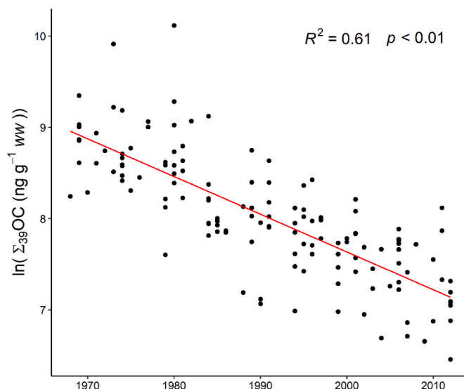
Fig. 2. Annual concentrations of the sum of 39 organochlorine (OC; list of compounds in section 2.5) in feather pools ( N = 135 ) from breeding pairs of adult white-tailed eagles ( Haliaeetus albicilla ) in Sweden in 1968–2012. Concentrations are natural log ( \ln ) transformed, and concentrations (filled dots) are calculated from a pool of feathers in which one pool represented a breeding pair. Number of feather pools analysed for pollutants were 1–9 per year, except in 1978, 1983, 1987, 1992–1993, and 1998, when feathers were not sampled. Estimate (red line) from the linear model investigating the temporal variations in OC concentrations is given in the supplementary information, Table S3.
