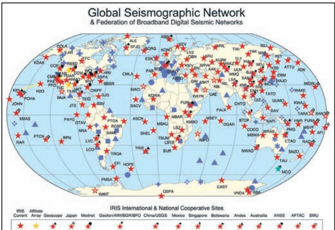
The Global Seismographic Network (GSN) consists of more than 125 GSN stations located around the world with near-uniform spacing. Map courtesy of the Global Seismographic Network (GSN), a cooperative scientific facility operated jointly by the Incorporated Research Institutions for Seismology (IRIS), the United States Geological Survey (USGS), and the National Science Foundation (NSF).
