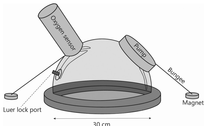
Fig. 2. Simplified sketch of the dome layout (not to scale).
