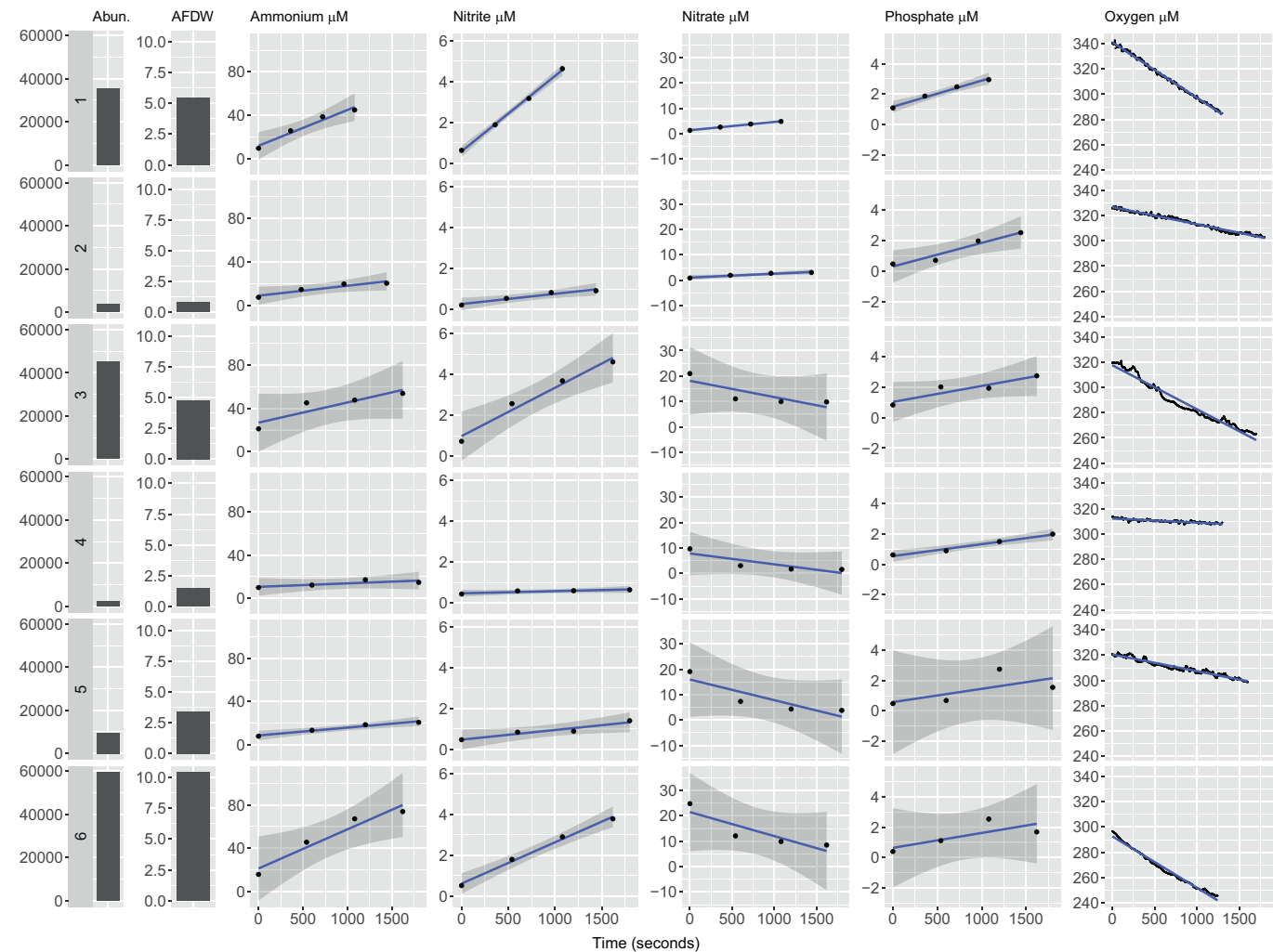
Fig. 5. Measured concentrations (µM) per sample (black dots) and modelled change during incubations (blue line) and 95% confidence intervals (grey ribbons). Rows: Sample ID, columns: 1 = abundance per sample, 2 = ash free dry weight per sample, 3 = ammonium (µM), 4 = nitrite, 5 = nitrate, 6 = phosphate, 7 = oxygen. Sample ID (left grey boxes) as presented in Table 1. (For interpretation of the references to colour in this figure legend, the reader is referred to the web version of this article.)
