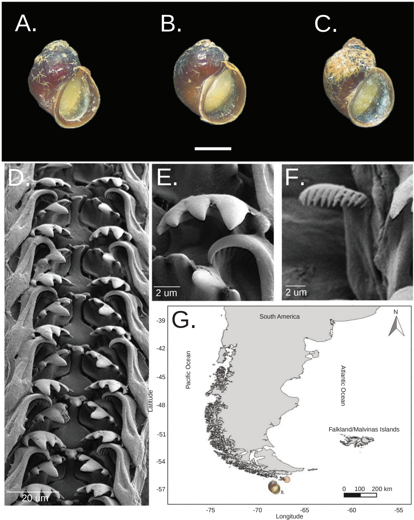
Figure 7. Laevitorina hicana , Hornos Island, southern South America. Scale bars: 1 mm unless specified otherwise. A–C, shell morphology and coloration of specimens collected from Hornos Island. D–F, radular morphology (SEM), showing a general view (D), lateral view (E), and outer marginal (F). G, distribution of L. hicana at Hornos Island, Cape Horn, southern South America.
