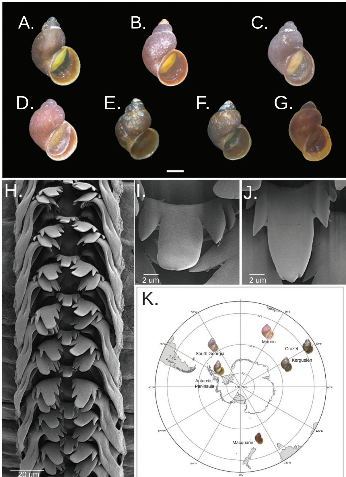
Figure 5. Laevilitorina venusta , Southern Ocean. Scale bars: 1 mm unless specified otherwise. A–G, variation in shell morphology and coloration of the species across its distribution in different provinces of the Southern Ocean. The specimens of L. venusta are from: Greenwich Island, South Shetland Islands, Antarctic Peninsula (A); Covadonga Bay, the Antarctic Peninsula (B); South Georgia (C); Marion Island (D); Crozet Island (E); Kerguelen Island (F); and Macquarie Island (G). H–J, radular morphology (SEM), showing a general view (H), rachidian (I), and rachidian from an individual from Antarctica showing small denticles (J). K, distributional pattern of L. venusta across the Southern Ocean.
