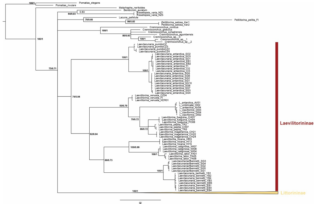
SI Figure 2: Phylogenetic reconstruction of the relationships among Littorinidae based on COI gene. Bayesian posterior probability (PP) and maximum likelihood bootstrap (ML) values are shown above and under the nodes.
