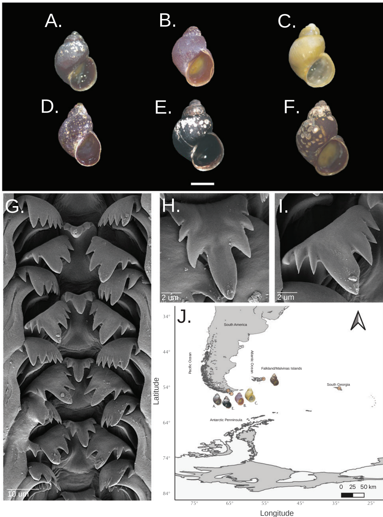
Figure 6. Laevivittorina caliginosa , Southern South America, South Georgia, and Falkland/Malvinas Islands. Scale bars: 1 mm unless specified otherwise. A–F, specimens of L. caliginosa from: Caleta Paula, Beagle Channel (A); Robalo Bay, Beagle Channel (B); Hornos Island (C); Puerto Williams, Beagle Channel (D); Ushuaia, Beagle Channel (E); and Falkland/Malvinas Islands (F). G–I, radular morphology (SEM), showing a general view (G), rachidian (H), and lateral view (I). J, distribution of L. caliginosa in the southern tip of South America, the Falkland/Malvinas Islands, and South Georgia.
