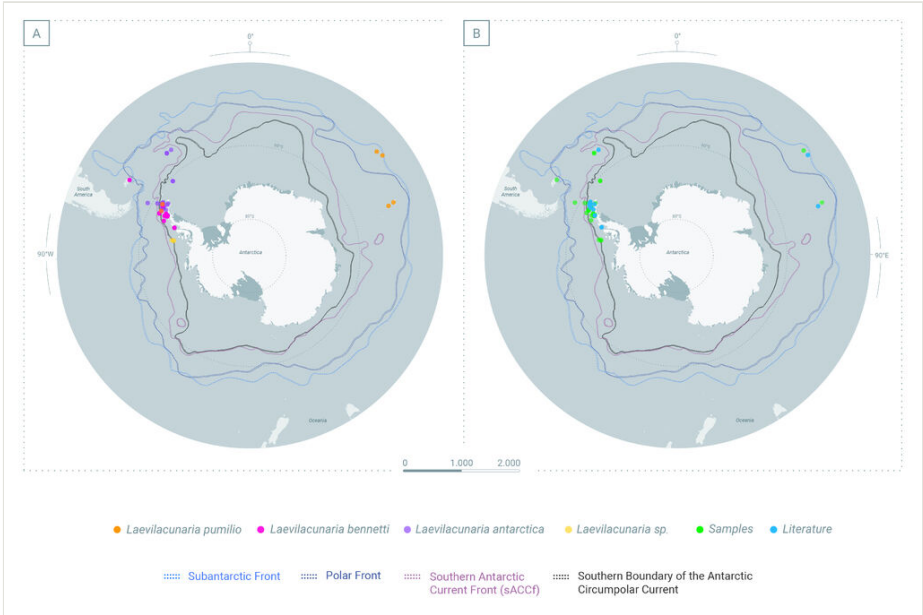
Figure 1. doi Distribution of all records of the genus Laevilacunaria in the Southern Ocean (SO). A Distribution of the three different species of Laevilacunaria in the SO; B Distribution of the specimen of the genus Laevilacunaria reported in the Southern Ocean showing the origin of the sources; literature and sampling.
