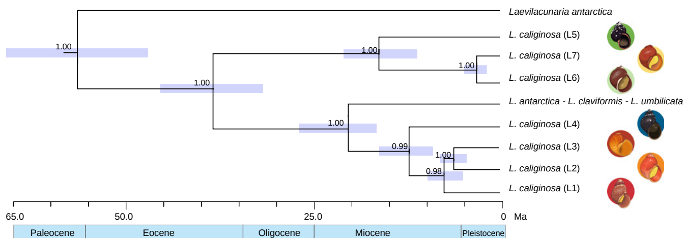
FIGURE 4 Divergence time estimations of Laevitorininae ( Laevitorina + Laevilacunaria ) based on mtDNA sequences using estimated calibrations by Reid et al. (2012). BPP values are indicated at nodes and shaded bars indicate 95% highest posterior density (HPD) intervals.
