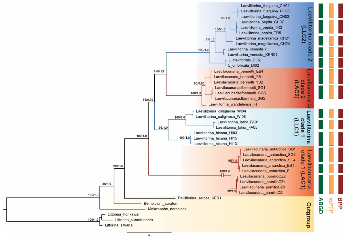
Figure 3. Phylogenetic reconstruction of the relationships among Laevilitorininae based on multilocus data (12S+16S+COI+28S), using the genus Pellilitorina , Bembicium , Melarihapse and Littorina as outgroups, showing
