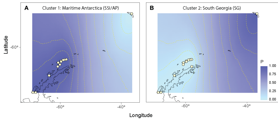
FIGURE 2 Spatial output from Geneland using Laevilacunaria antarctica populations. White circles indicate the relative positions of the sampling localities across maritime Antarctica and South Georgia. Darker and lighter shadings are proportional to posterior probabilities of membership to particular genetic cluster ( A = maritime Antarctica and B = South Georgia). Posterior probabilities were plotted against the shapefile of the Antarctic coastline available in GEODas (NOAA) and filtered using GEODas Coastline Extractor v.1.1.3.1 ( https://www.ngdc.noaa.gov/mgg/geodas/geodas.html ).
