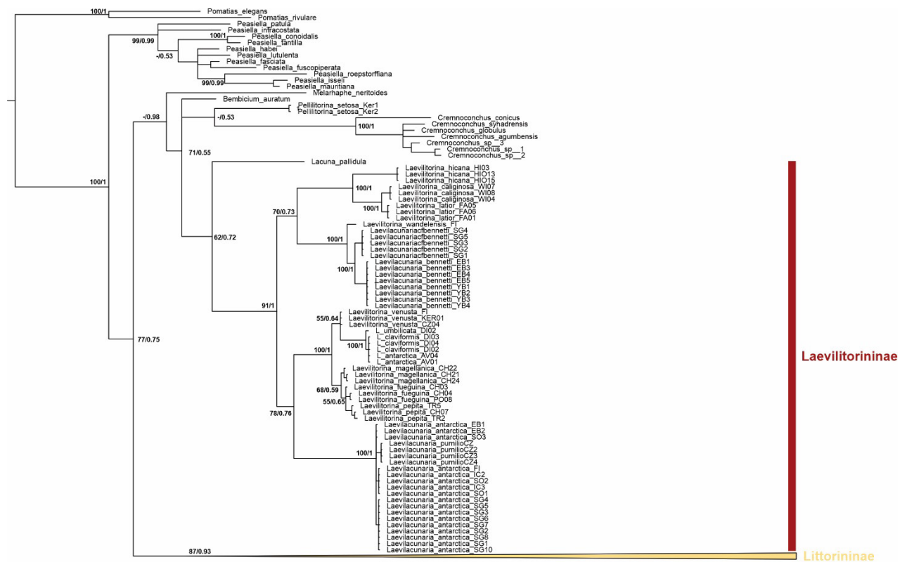
SI Figure 1: Phylogenetic reconstruction of the relationships among Littorinidae based on 12S gene. Bayesian posterior probability (PP) and maximum likelihood bootstrap (ML) values are shown above and under the nodes.
