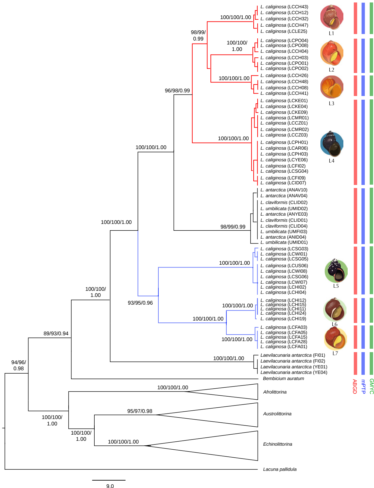
FIGURE 3 Bayesian maximum cladocredibility tree of Littorinidae relationships based on multi-locus data with special emphasis on Laevilitorina ( Laevilitorina & Laevilacunaria ) populations collected from around the Southern Ocean. The lineages (L1–L7) recorded within the nominal species L. caliginosa are shown. Red and blue rectangles indicate the paraphyletic groups of Laevilitorina lineages found within L. caliginosa . Bootstrap support (BS) values (MP and ML) and Bayesian posterior probabilities (BPP) are shown above the nodes (in that order).
