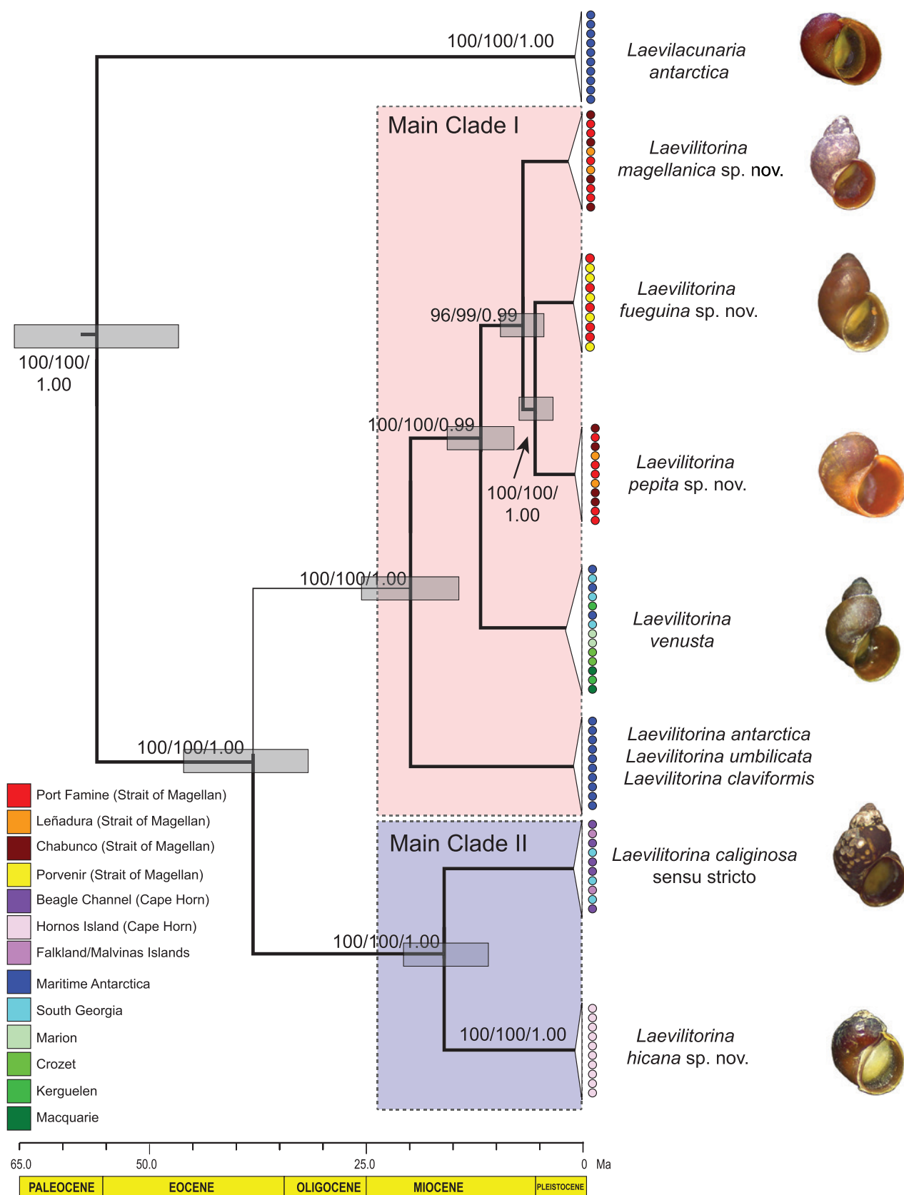
Figure 1. Bayesian maximum credibility tree of Laevilitorininae ( Laevilitorina and Laevilacunaria ) relationships based on mitochondrial DNA (COI) and nuclear DNA (28S rRNA) sequences. Bootstrap support values for maximum parsimony, maximum likelihood, and Bayesian posterior probabilities are shown above the nodes (in that order). Divergence time estimations were performed based on mitochondrial DNA sequences using a calibrated littorinid phylogeny following Reid et al. (2012).
