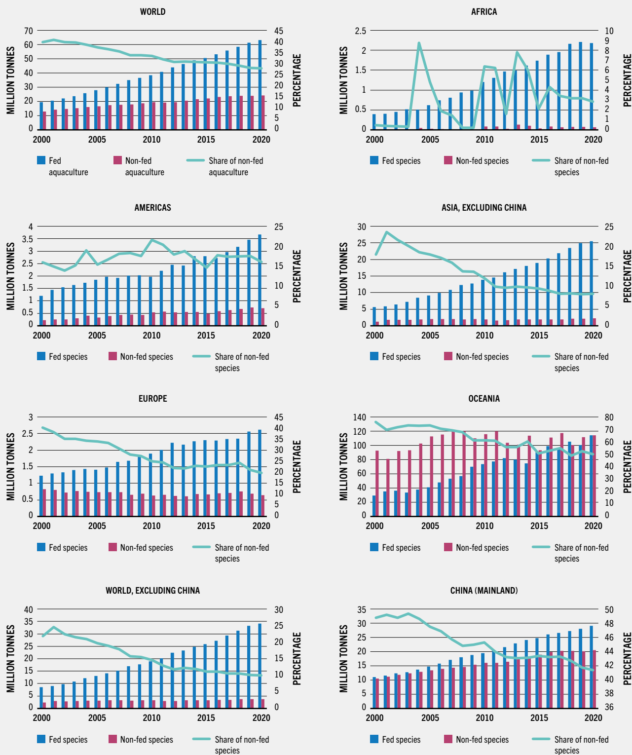
FIGURE 21 FED AND NON-FED AQUACULTURE PRODUCTION OF ANIMAL SPECIES BY REGION, 2000–2020
