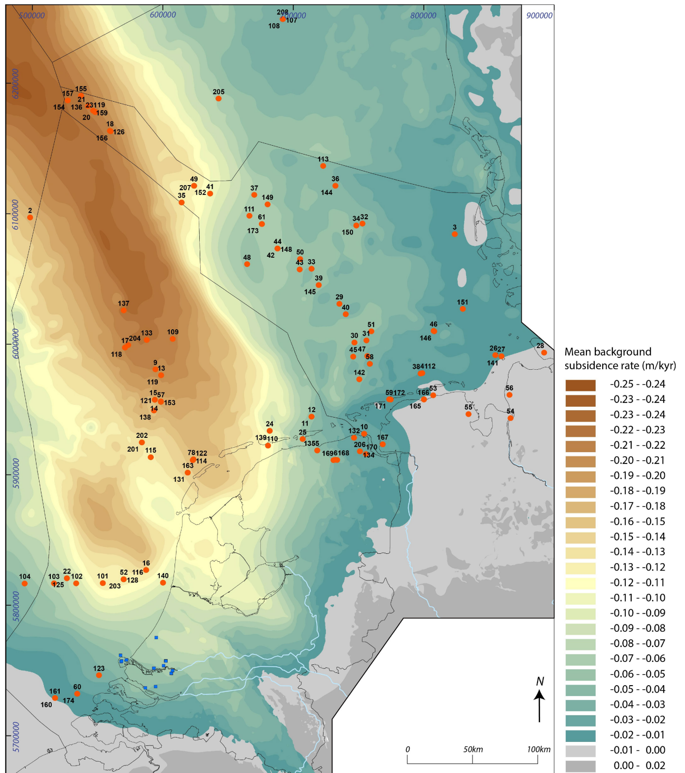
Extended Data Fig. 3 | Mean background subsidence rate (m/kyr) over the last 1.8 Ma for the North Sea Basin. The subsidence rates and associated spatial pattern are not related to GIA processes. Instead, they are a cumulative
