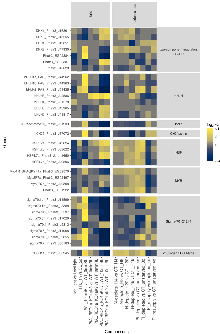
Figure 3. RNA-Seq heatmaps of twocomponents regulators and transcription factors. Heatmap showing gene expression differences in light and nutrient stress experiments for different genes of interest. “HighLight versus LowLight” compares low light and high light acclimated wild-type (WT) strains (Agarwal et al., 2022). “sFL_1h versus CL_5d” compares strains acclimated to constant light conditions to severe light fluctuation conditions (Zhou et al., 2022). “WT10minBL versus WT0minRL” compares WT strains under red light (RL) and 10 min after a shift to blue light (BL); In samples “PtAUREO1a_KO1aK8 versus WT_0minRL”, “PtAUREO1a_KO1aK9 versus WT_0minRL”, “PtAUREO1a_KO1aK8 versus WT_10minBL” and “PtAUREO1a_KO1aK8 versus WT_10minBL”, Aureo1a knockout K8 and K9 strains are compared to WT under RL, and after a 10 minutes shift to BL (Mann et al., 2020). “N-deplete versus CT” compares nitrate-deplete and control samples 4, 8, and 20 h after transfer to nitrogen-replete medium (Matthijs et al., 2016; Matthijs et al., 2017). “N-deplete_H48 versus CT_H48” compares nitrogen-free and nitrogen-replete samples after 48 h of treatment (Levitani et al., 2015). “Pi-depleted versus CT_unstarved_4d” and “Pi_depleted versus CT_unstarved_8d” compare control samples and cultures without phosphate supplement during 4 and 8 days. “Pi_resupply versus depleted_4d” and “Pi_resupply versus CT_unstarved_4d” compare samples with phosphate re-supplementation after 4 days of starvation (Cruz de Carvalho et al., 2016). *Based on the prediction supported by the database, these genes are localized in the plastid.
