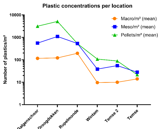
Figure 2. Plastic concentrations in number of items per m 2 across the sampled locations during the PLASTFLOW project.
