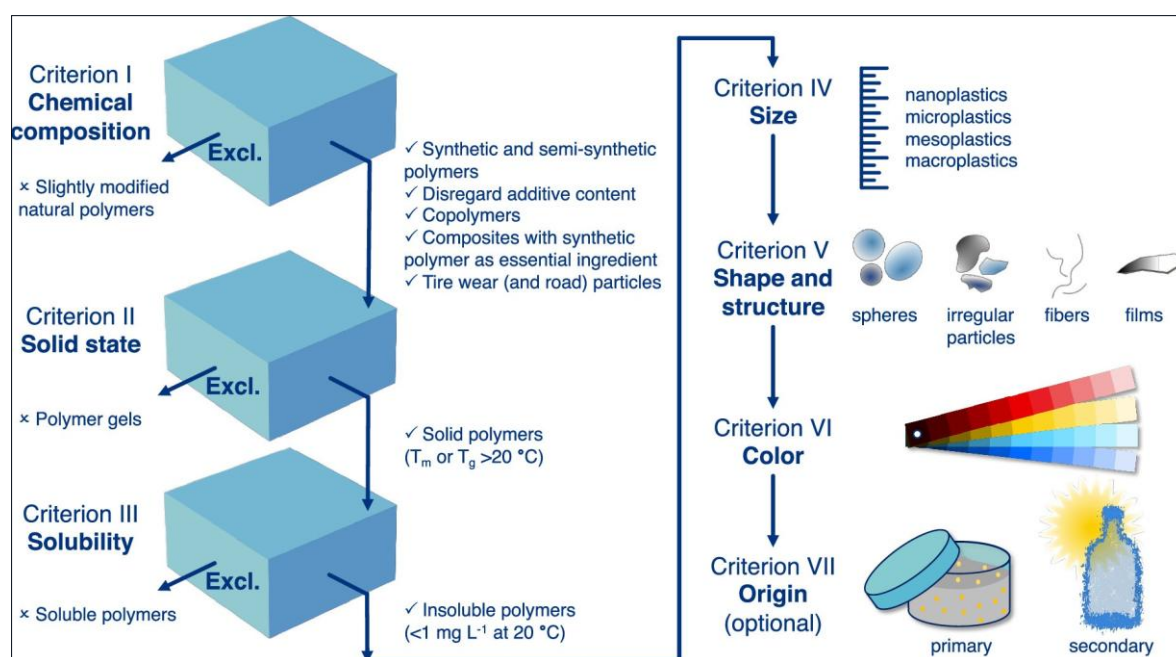
Figure 1.6. Framework for the definition and categorization of plastic particles proposed by Hartmann et al. (2019), based on seven hierarchical criteria: chemical composition, solid state, insolubility, size, shape and structure, color, and (optionally) origin.
