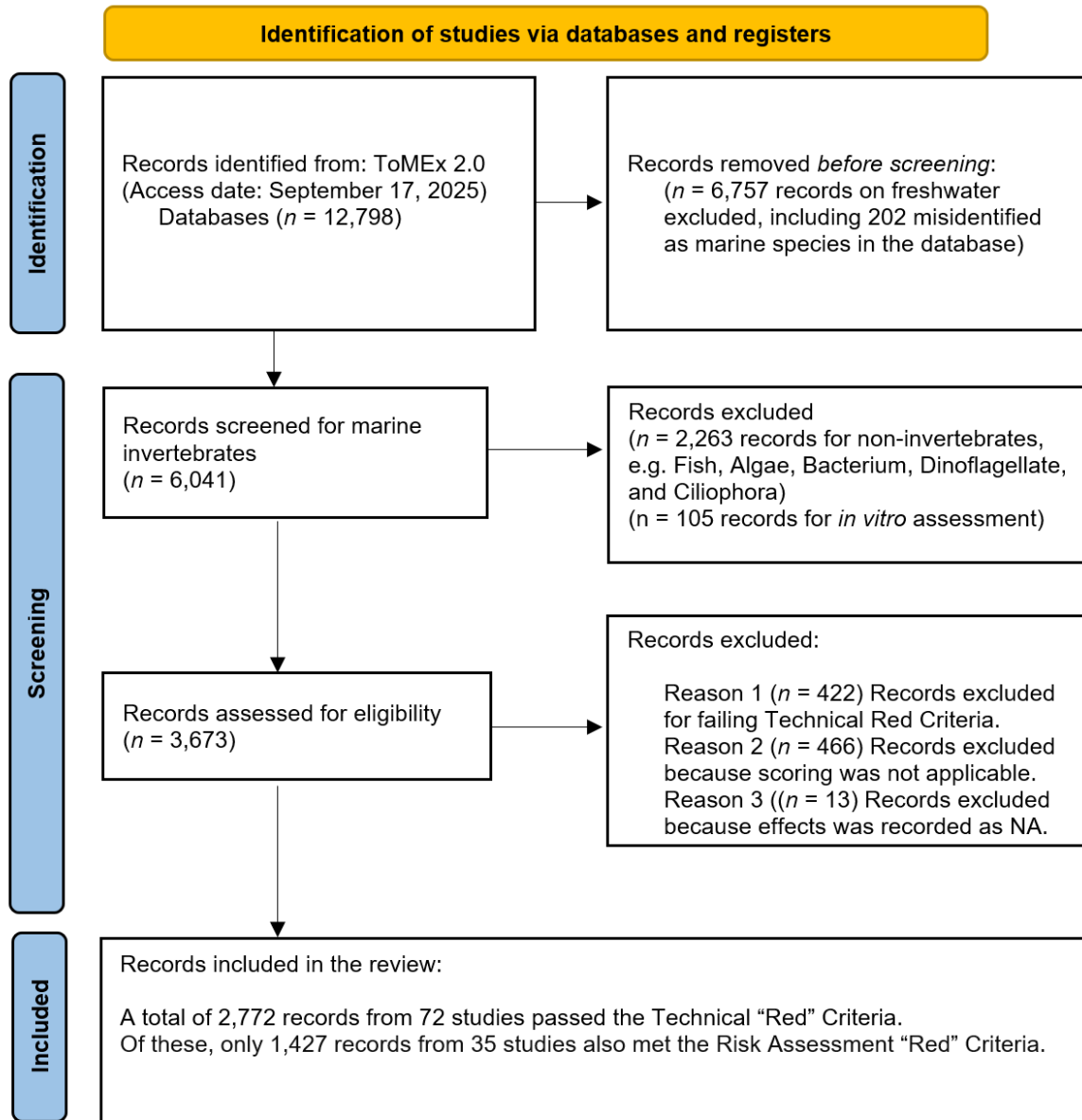
Figure A2.1. Flowchart of the selection process following the Preferred Reporting Items for Systematic Reviews and Meta-Analyses (PRISMA) guidelines.
