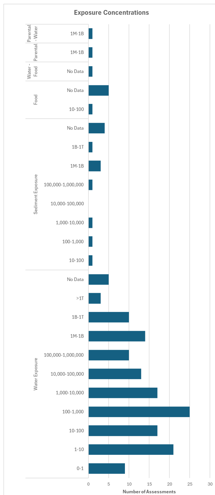
Figure 2.3. Distribution of particle exposure concentrations assessed in in vivo MNP toxicity studies ( n = 72 ) on marine invertebrates. Exposure routes include sediment (particles/kg dry weight) and water, along with other exposure pathways (particles/mL). 'No Data' indicates the absence of explicitly reported concentration values in the reviewed studies.
