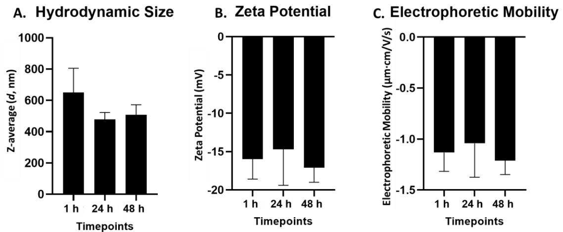
Figure A3.2. Hydrodynamic size (A), zeta potential (B), and electrophoretic mobility (C) of aged PET MNPs in artificial seawater (pH 8.1) measured over time (1 h, 24 h, and 48 h) using Dynamic Light Scattering. Data are expressed as mean \pm standard deviation ( n = 3 ) for each time point.
