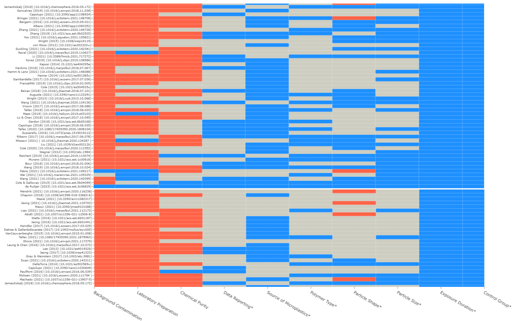
Figure A2.3. Heatmap showing the scoring of individual MNP toxicity studies (n = 72) across technical criteria. Colors represent scores: Adequate (blue, score = 2), Adequate (orange, score = 1), Inadequate (grey, score = 0).
