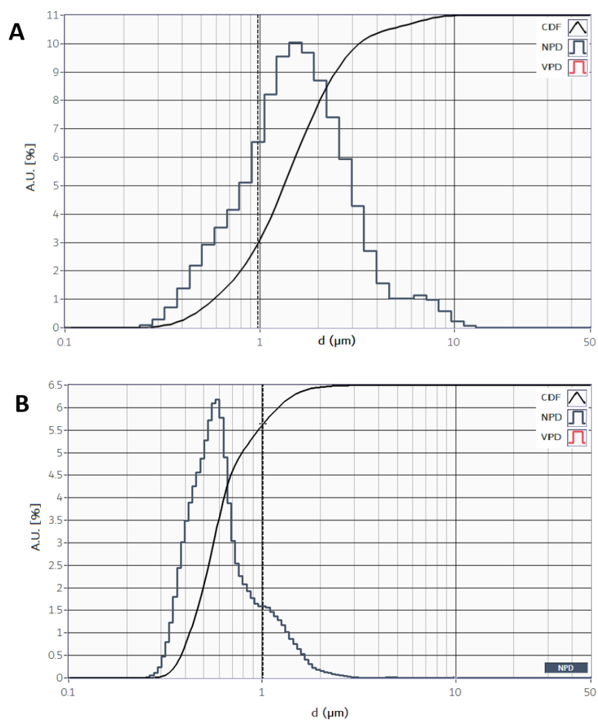
Figure A4.1. Particle size distribution analysis of aged PET MPs ( Panel A ) and NPs ( Panel B ) using Single Particle Extinction and Scattering (SPES). The number-based particle size distribution is shown together with the corresponding cumulative distribution function (CDF) as a function of particle diameter ( d ).
