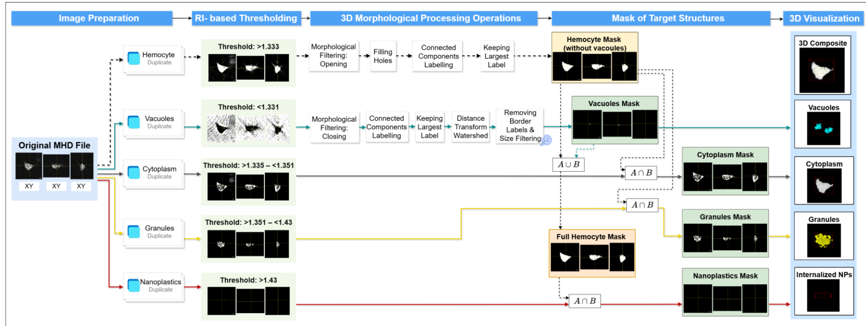
Figure 5.2. Schematic overview of the image-processing pipelines applied to 3D refractive-index (RI) tomograms. The workflow was implemented in ImageJ-Fiji (Version 1.54p) using customized macro-scripts that called various functions, primarily from the MorphoLibJ and 3D Viewer plugins (cf. text for details). Key steps include spatial calibration, thresholding, 3D morphological processing, image calculator operations (union: \cup and intersection: \cap ) and 3D visualization and quantitative analyses of segmented cell structures. Supplementary Figures A5.9 and A5.10 provide representative examples of each step, illustrating encountered situations for hemocytes featuring or not internalized nanoplastic particles, respectively.
