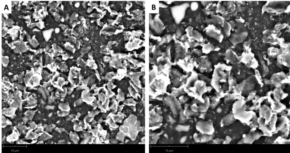
Figure A4.3. Scanning electron microscopy (SEM) images of the aged PET micro- and nanoplastic particles (MNPs) captured using a Phenom™ ProX Desktop SEM system. The images, taken at magnifications of (Panel A) 4400x and (Panel B) 7000x, reveal the weathered and irregular shapes of the particles with evident heterogeneous sizes.
