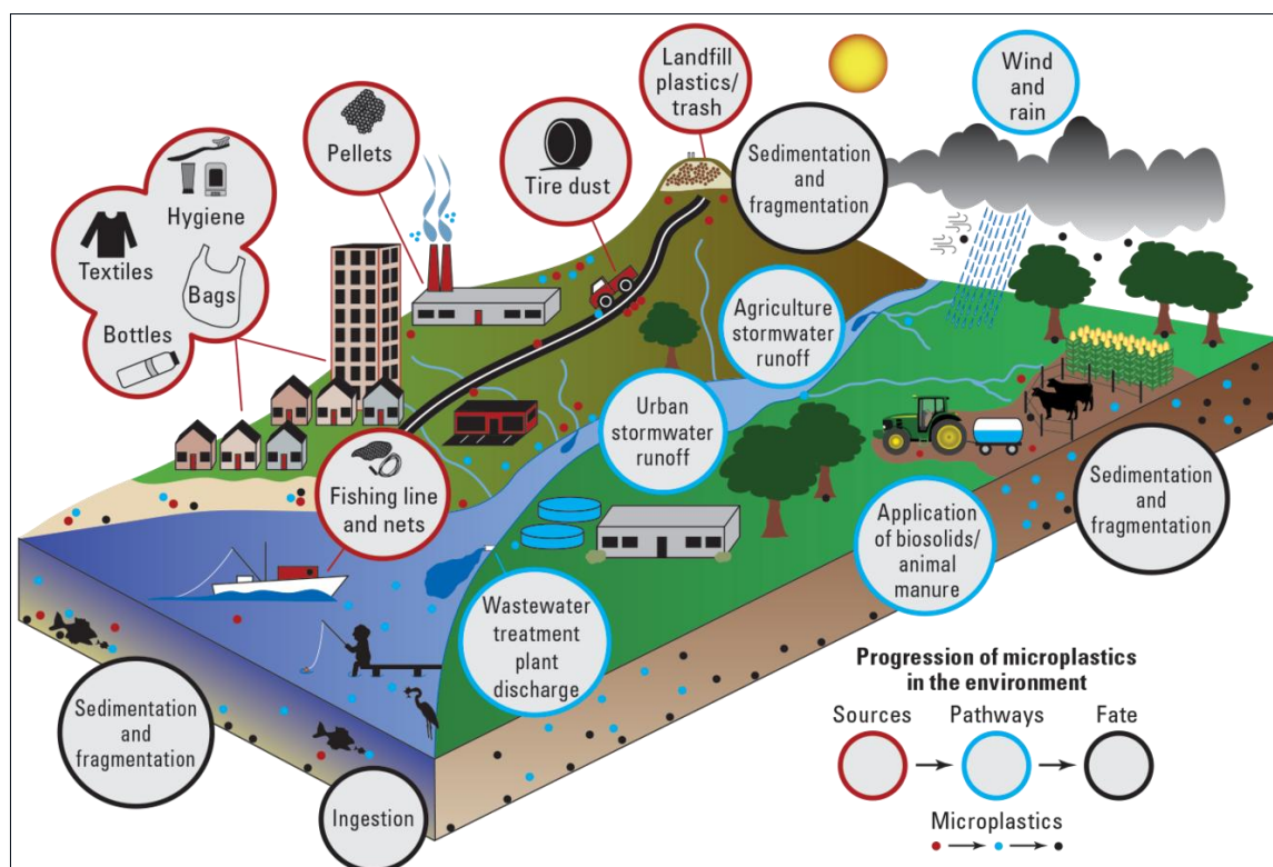
Figure 1.5. A conceptual diagram illustrating the major sources, environmental pathways, and fate of plastic particles in the environment. Adapted from: Environmental Health Program of USGS (2023).
