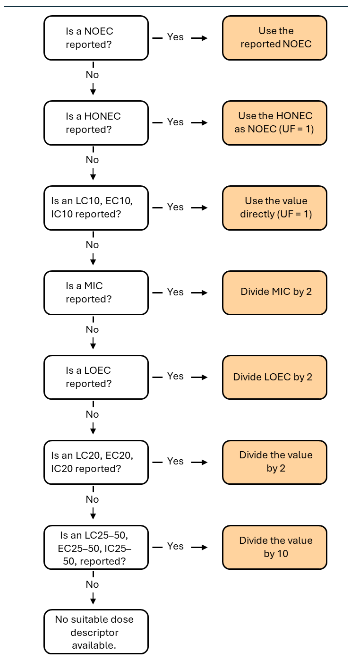
Figure A2.5. Decision tree used for standardizing effect concentrations to no-observed-effect concentrations (NOECs) in MNP toxicity studies. The figure illustrates the hierarchical approach and associated uncertainty factors (UFs) applied to convert various reported dose descriptors to NOECs, based on established reference (Wigger et al., 2020). Abbreviations: HONEC, highest observed no-effect concentration; MIC, minimum inhibitory concentration; LOEC, lowest observed effect concentration; LC, lethal concentration; EC, effective concentration; IC, inhibitory concentration; UF, uncertainty factor.
