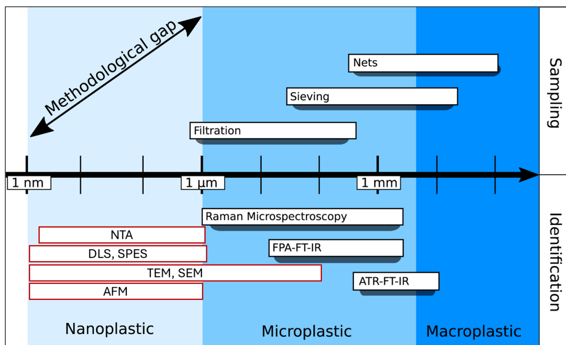
Figure 1.8. Overview of current analytical methodologies for sampling and identifying plastic particles across size ranges, highlighting a critical methodological gap for nanoplastic particles ( <1\ \mu\text{m} ). Techniques indicated in red boxes are mainly applicable in controlled or clean matrices and have limited applicability for complex biological or environmental samples. Abbreviations: NTA, nanoparticle tracking analysis; DLS, dynamic light scattering; SPES, single-particle extinction and scattering; TEM, transmission electron microscopy; SEM, scanning electron microscopy; AFM, atomic force microscopy; FPA-FT-IR, focal plane array Fourier-transform infrared spectroscopy; ATR-FT-IR, attenuated total reflectance Fourier-transform infrared spectroscopy. Adapted from: Schwaferts et al. (2019).
