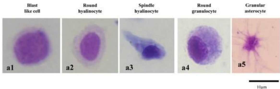
Figure A5.16. Morphological reference images used for the identification of hemocyte subpopulations: blast-like cells (a1), round hyalinocytes (a2), spindle hyalinocytes (a3), round granulocytes (a4), and granular asterocytes (a5). Scale bar: 10 \mu\text{m} . Adapted from Ray et al., 2013.
