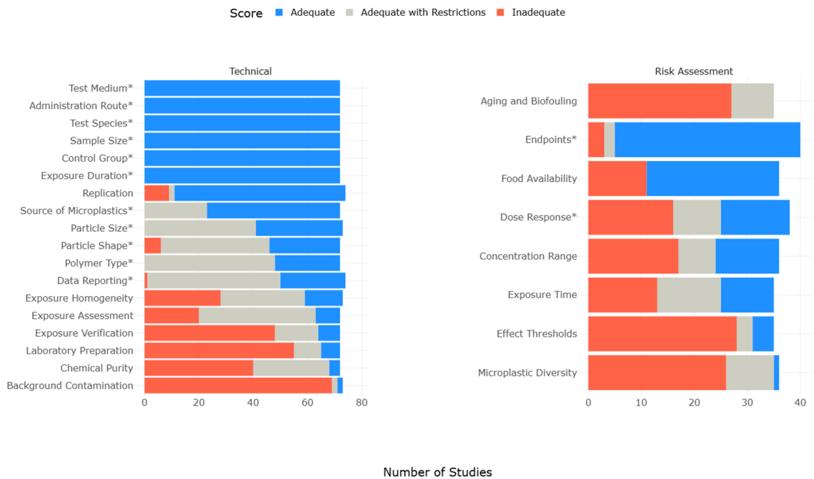
Figure A2.2. Quality scores of MNP toxicity studies in ToMEx 2.0 that met the Technical ( n = 72 ) and Risk Assessment (subset, n = 35 ) Red Criteria. Bar plot depicting the number of studies rated as Adequate (blue, score 2), Adequate with Restrictions (gray, score 1), or Inadequate (red, score 0) across assessed criteria. 'Red Criteria', indicated by an asterisk (*), denote the minimum requirements for technical and risk assessment, as defined by Mehinto et al. (2022).
