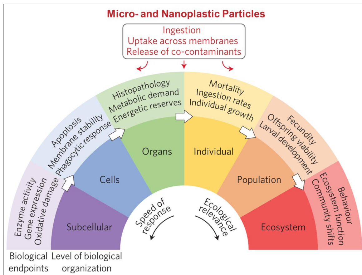
Figure 1.13. Framework illustrating the potential biological impacts of micro- and nanoplastic particle exposure across different levels of biological organization, from subcellular responses to ecosystem-level effects. Adapted from: Galloway et al. (2017).
