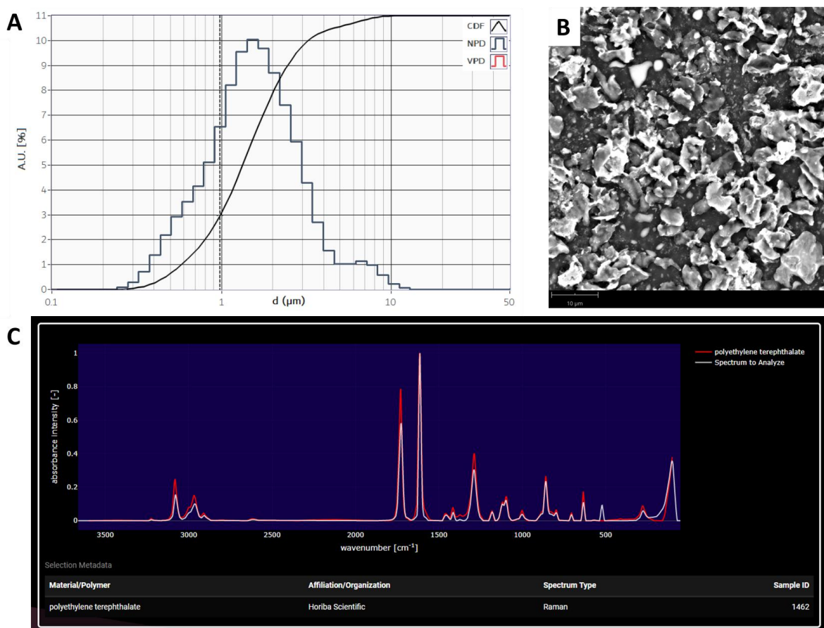
Figure A3.1. Particle size distribution (A), shape (B), and polymer type (C) of aged PET MNPs analyzed using Single Particle Extinction and Scattering (SPES) technique (ClassizerONE, S1.4.34, EOS), scanning electron microscopy (SEM, Phenom™ ProX) and Raman spectroscopy with Open Specy reference library. Panel A displays the particle size distribution of the aged PET MNPs measured by SPES. The number-based particle size distribution is shown together with the corresponding cumulative distribution function (CDF) as a function of particle diameter (d). Panel B SEM images of the particles captured using a Phenom™ ProX Desktop SEM system. The image, taken at magnifications of 4400x, reveals the weathered and irregular shapes of the particles with evident heterogeneous sizes. Panel C shows the Raman spectrum of the aged PET MNP sample acquired using an inVia™ Qontor® confocal Raman microscope (Renishaw, Wotton-under-Edge, UK) equipped with a 785 nm excitation laser and a 20× objective. PET suspensions were diluted in ethanol (1:3, v/v), deposited onto a silicon wafer, and measured in the dry state after solvent evaporation. The instrument was operated at 10% laser power, with an accumulation time of 1 s, averaging 5 accumulations. The spectrum was compared against the Open Specy reference library, confirming the material as PET with a 0.97 match score relative to the reference spectrum.
