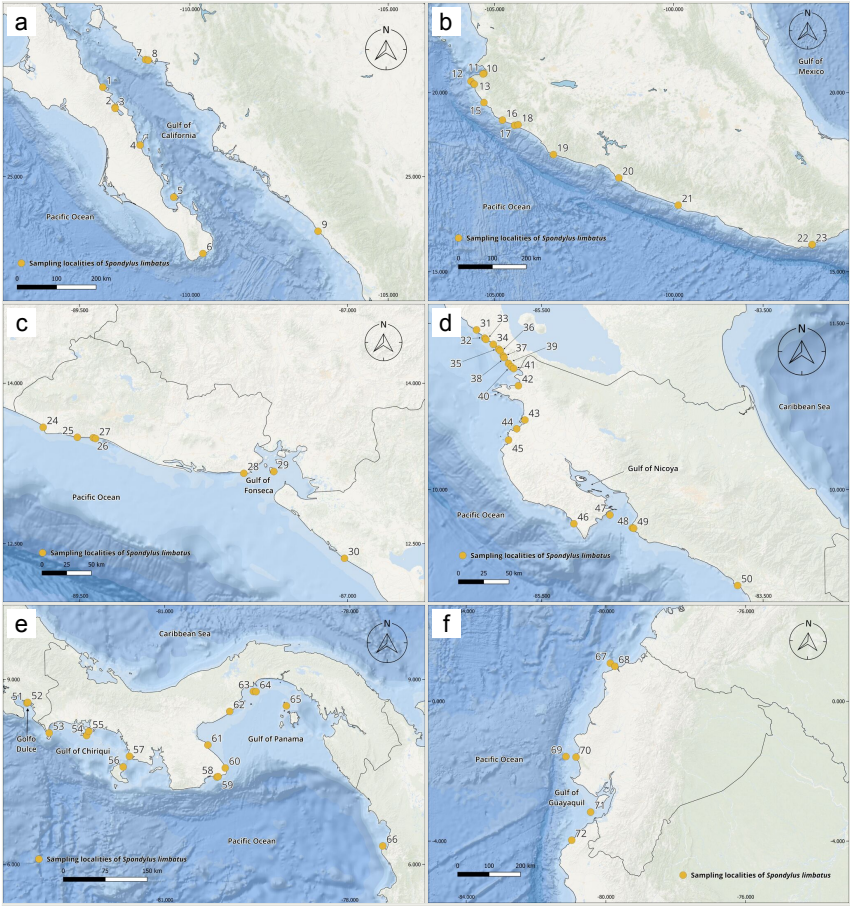
Figure 2. Sampling localities of Panamic Province specimens. Maps were created in QGIS using the ESRI Ocean Basemap. Yellow dots indicate sampling localities (Table 1): a: Gulf of California; doi b: Central Mexico; doi c: El Salvador-northwestern Nicaragua; doi d: South-western Nicaragua-Costa Rica; doi e: Southern Costa Rica-northwestern Colombia; doi f: Ecuador and northern Peru. doi
