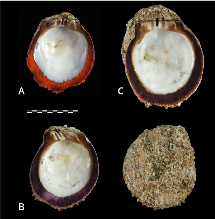
Figure 6. doi Variation in colouration along the inner margin of Spondylus limbatus : (A) orange specimen, Islote de Playa Hermosa (ID S044); (B) purple specimen (internal and external views), Cuajiniquil (ID S153); (C) reddish-brown specimen, El Ciruelo (ID S214).
