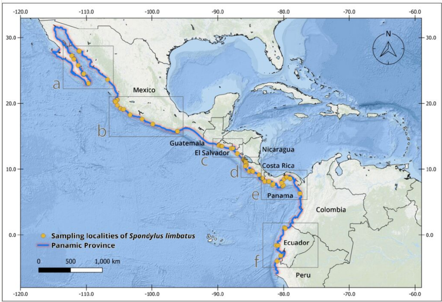
Figure 1. doi Geographical distribution of sampling localities of specimens from the Panamic Province. Maps were created in QGIS using the ESRI Ocean Basemap. Yellow dots indicate sampling localities.
