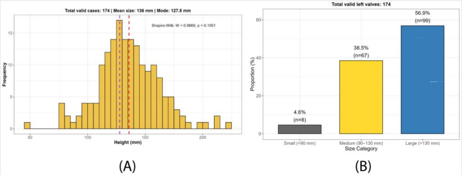
Figure 7. doi Frequency and size distribution of left valves in the collection: (A) Frequency distribution of left valve height in Spondylus limbatus specimens; (B) Size-class distribution of left valve specimens in the reference collection.
