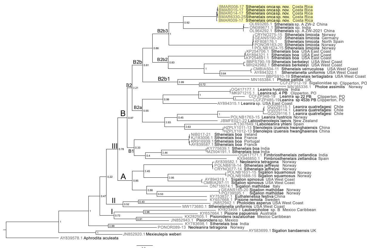
Figure 2. Bayesian phylogenetic tree of the family Sigalionidae based on COI sequences. Node support values are posterior probabilities. Clade labels are referred to in the text.
