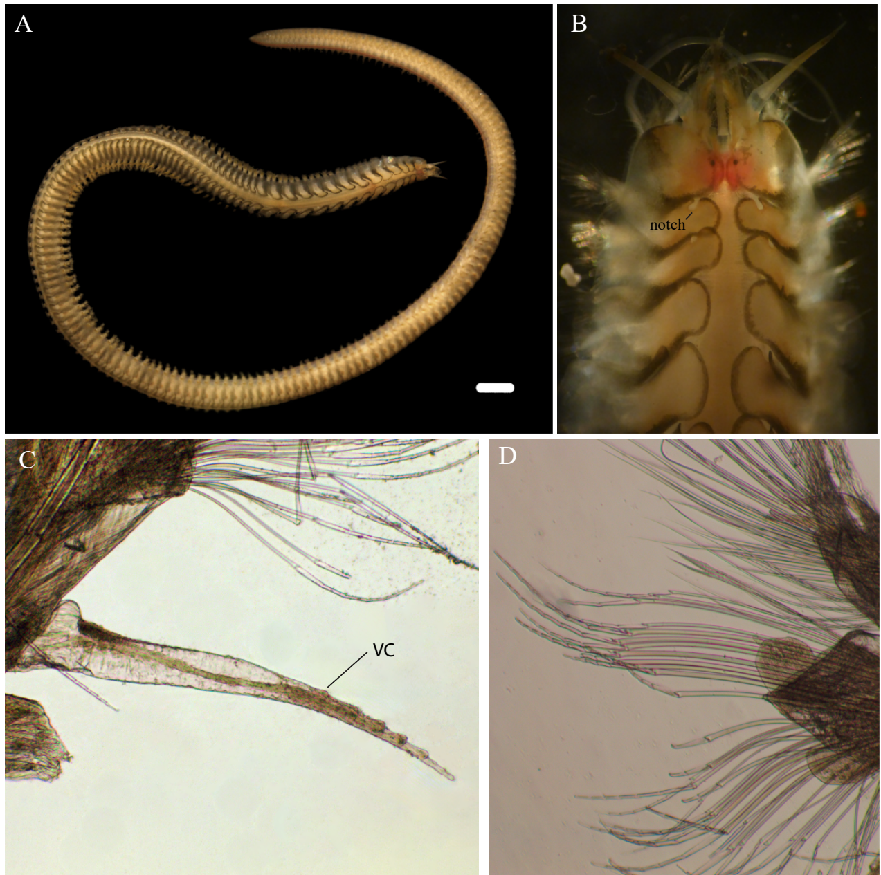
Figure 4. Sthenelais onca sp. nov. paratypes (MZ-UCR 387-02, 387-08). A. Paratype MZ-UCR 387-02, complete specimen; B. Anterior region showing live coloration and the elytral notch; C. Paratype MZ-UCR 387-08, detail of ventral cirrus; D. Paratype MZ-UCR 387-08, median chaetigers. The lower group of neurochaetae corresponds to compound falcigers with smooth shafts. Abbreviations: VC = ventral cirrus. Scale bar: 1 mm ( A ).
