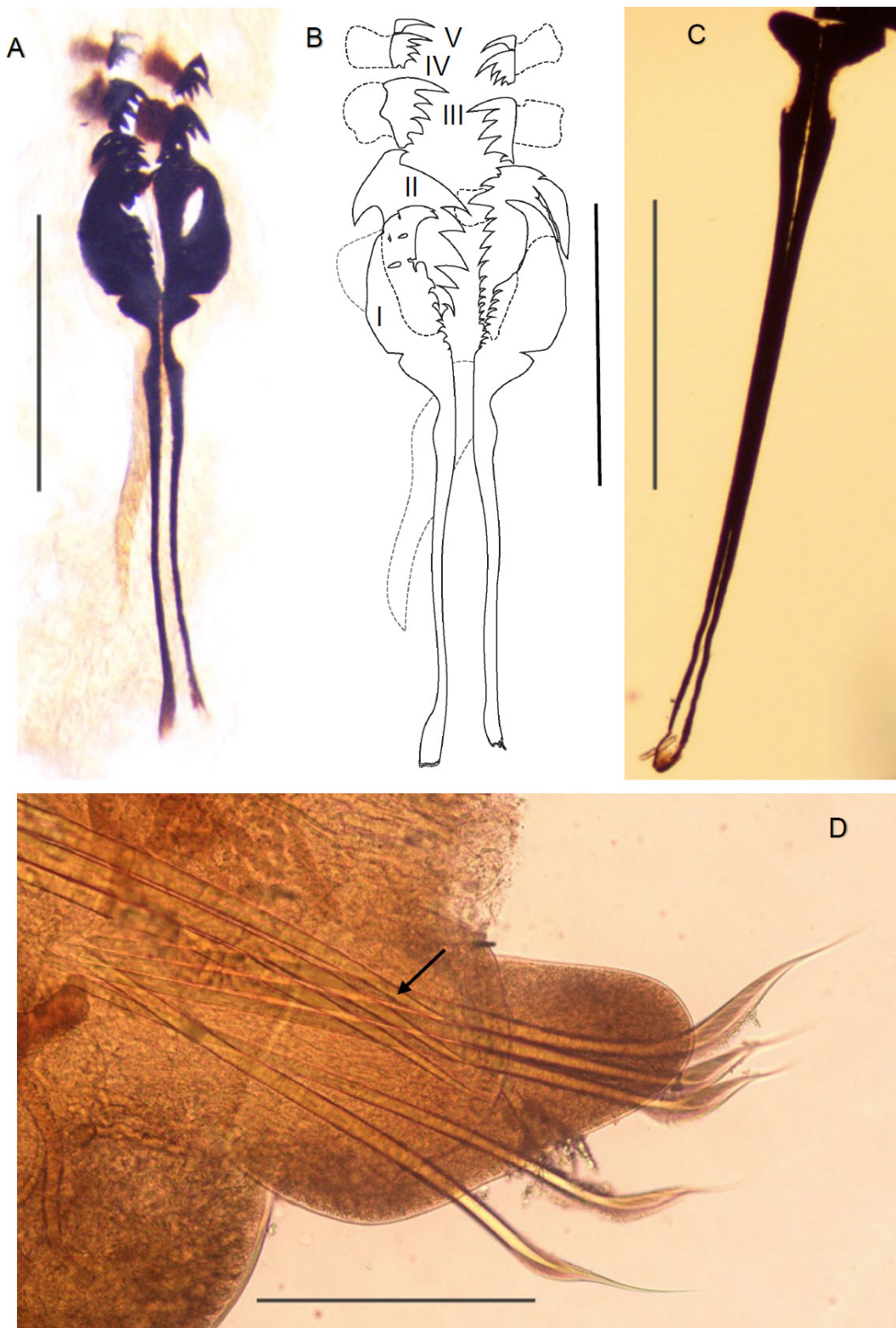
Figure 4. Arabella gouqi sp. nov. holotype CMSTT7 (A, B), paratype CMSTg13 (C), and paratype CMSTT4 (D). A. Maxillae (including ventral and dorsal carriers); B. Maxillae I–V; C. Dorsal carriers; D. Right parapodium 23 (arrow pointing to a notoacicula). Scale bars: 5 mm (A, C); 4 mm (B); 2.5 mm (D).
