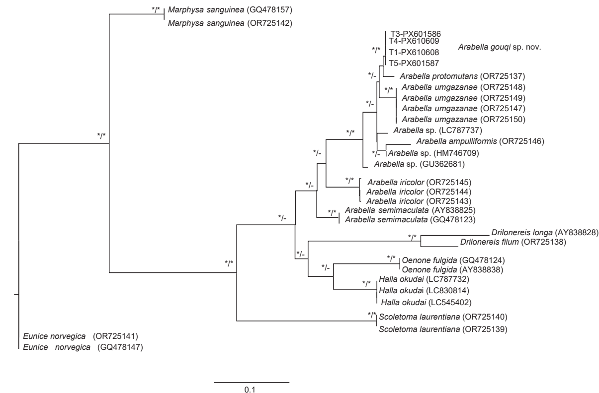
Figure 6. Maximum likelihood (ML) tree based on 16S rDNA sequences of Arabella species from different localities. Asterisks (*) at nodes indicate clades with \geq 95\% bootstrap values. The scale bar represents substitutions per site.
