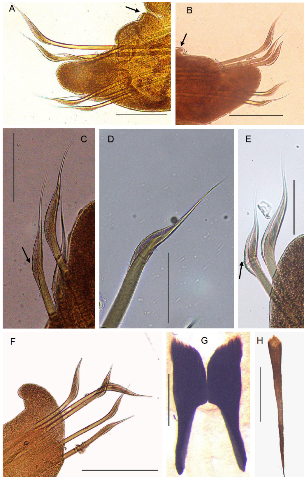
Figure 3. Arabella gouqi sp. nov. holotype CMSTT7 (F), paratype CMSTT4 (B, D, E), paratype CMSTT5 (H), and paratype CMSTT6 (A, C, G). A. Left parapodium 22 (arrow pointing to a notopodial cirri); B. Right parapodium 24 (arrow pointing to a notopodial cirri); C. Right parapodium 22 (arrow pointing to the ventralmost chaetae); D. Ventralmost chaetae, right parapodium 23; E. Dorsal and mediodorsal chaetae, left parapodium 25 (arrow pointing to coarsely serrated); F. Right parapodium 37; G. Mandibles; H. Ventral carrier. Scale bars: 8 mm (A, B); 2.8 mm (C, F); 1 mm (D, E); 3 mm (G, H).
