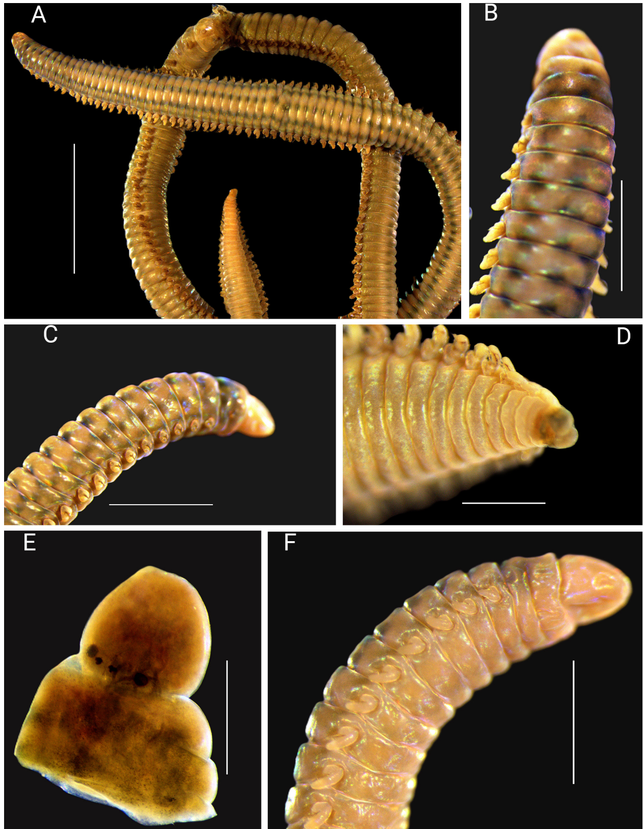
Figure 2. Arabella gouqi sp. nov. holotype CMSTT7 (F), paratype CMSTT6 (A), paratype CMSTT4 (B, E), paratype CMSTT5 (C) and paratype CMSTT1(D). A. Complete body; B. Body, anterior dorsal view; C. Anterior, dorsolateral view; D. Pygidium ventrolateral view; E. Prostomium with four eyes; F. Anterior body, ventral lateral view. Scale bars: 7 mm (A); 4 mm (B–D); 12 mm (E); 15 mm (F).
