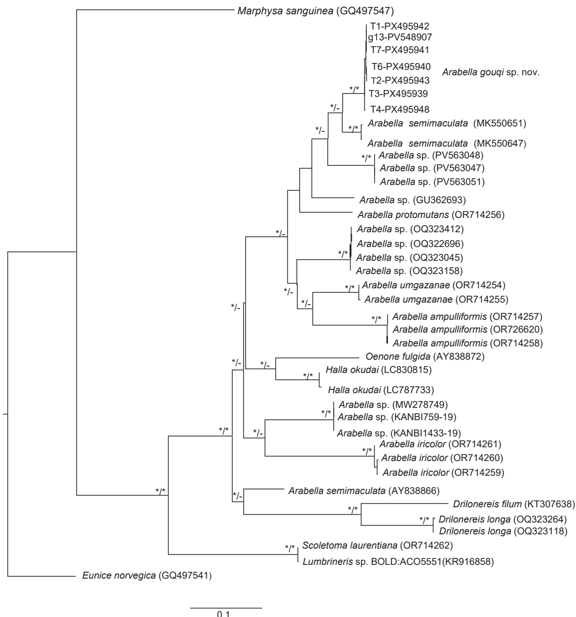
Figure 5. Maximum likelihood (ML) tree based on COI sequences of Arabella species from different localities. Asterisks (*/*) at nodes indicate clades with \geq 95\% bootstrap values. The scale bar represents substitutions per site.
