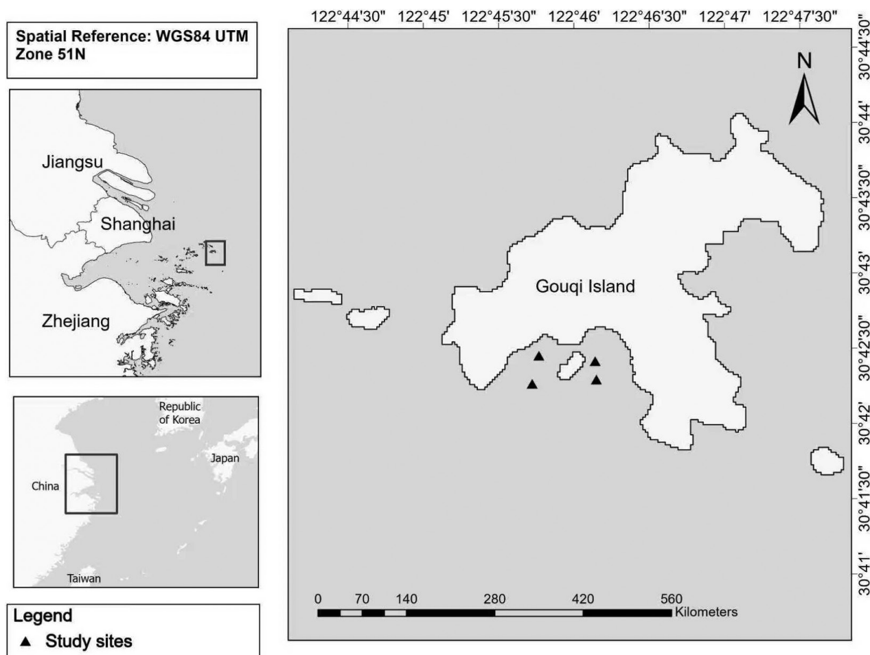
Figure 1. Sampling sites of specimens of Arabella gouqi sp. nov. off the coast of Gouqi Island, Zhejiang, China.
