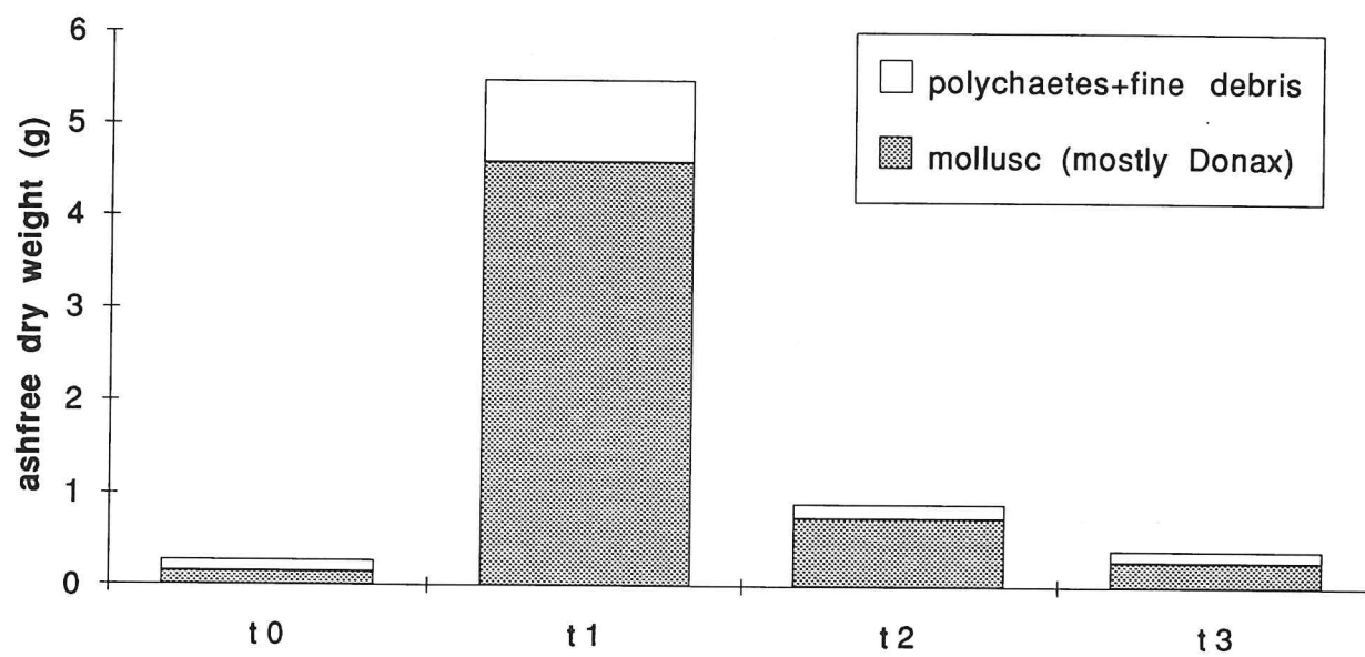
Fig. 3. Total stomach content (g ash free dry weight) of 30 dab ( Limanda limanda ) caught in the 3-m beam trawl, 12 hours before trawling ( t_0 ), immediately after trawling ( t_1 ), 12 hours after trawling ( t_2 ), and 24 hours after trawling ( t_3 ) (Vlieland study).
