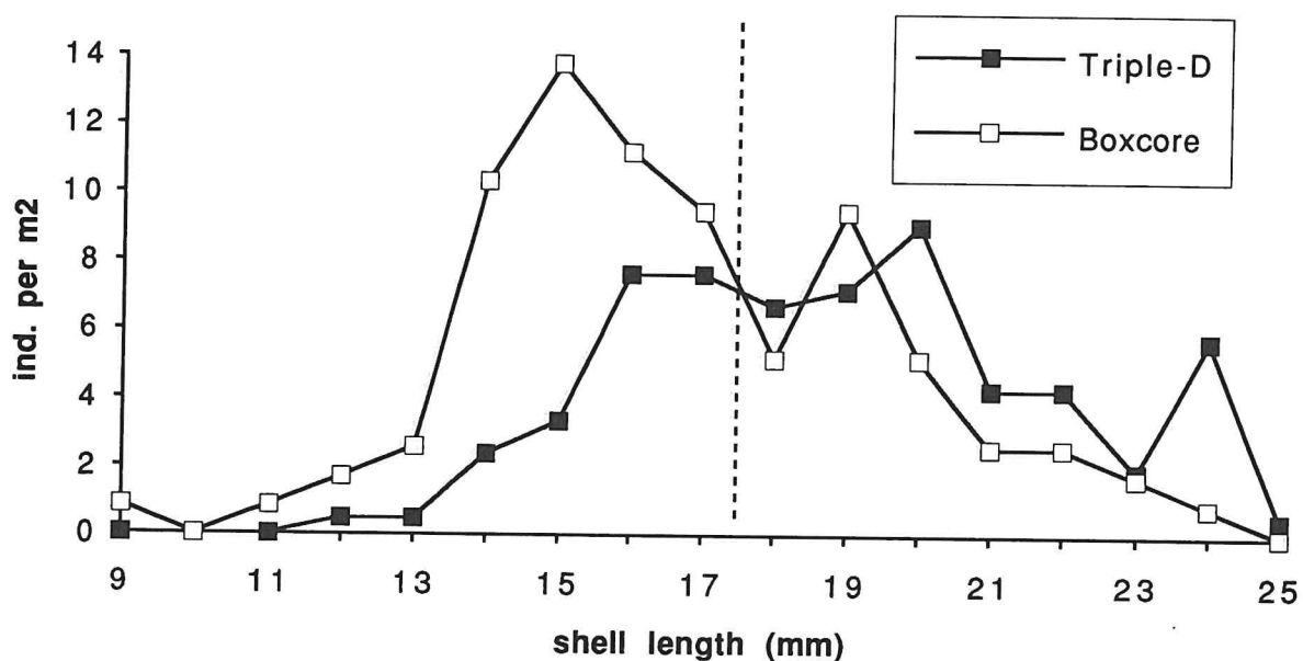
Fig. 2. Length distribution of Macoma balthica ( n \cdot m^{-2} ) from the box corer samples ( n = 91 from 14 grabs covering 1 m^2 ) and Triple-D (based on a subsample of 129 animals from 3 hauls covering 140 m^2 ). The dotted line indicates the length class below which it is possible to escape through the meshes of the dredge. Length classes to the left of this line were not taken into account for testing the Triple-D.
