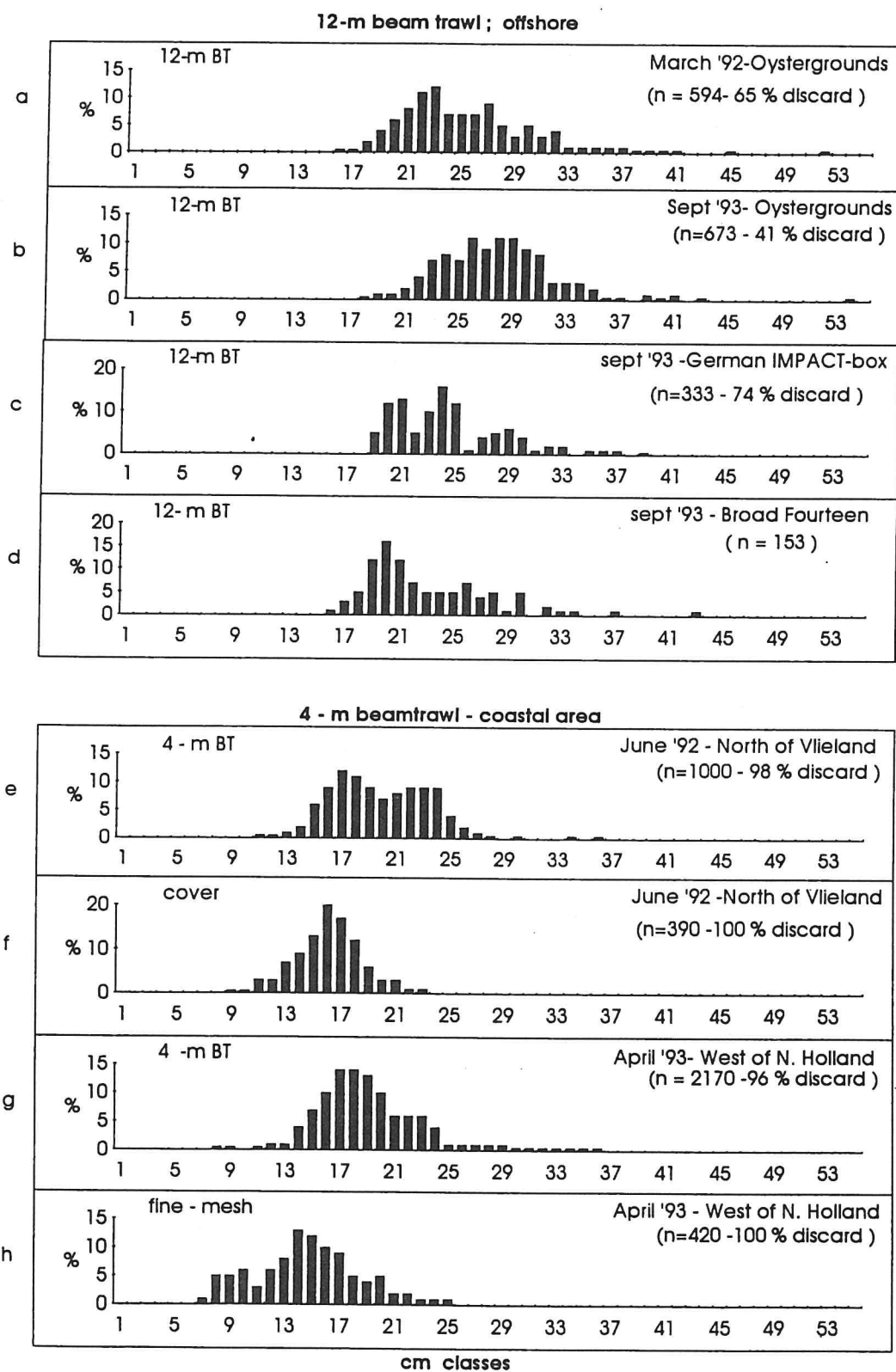
Figure 3. The length frequency distribution of plaice ( Pleuronectes platessa ). Catches with 12-m beam trawls (12mBT) offshore (a-d) and 4-m beam trawls (4mBT) in coastal areas (e,g) compared with catches in fine-meshed cod-end covering net (cover,f) or fine-meshed trawl (h).
