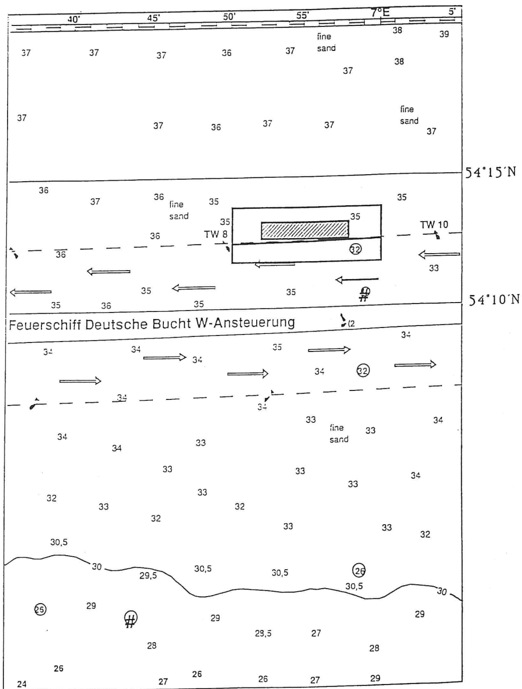
Fig. 2. The IMPACT box area 20 nm west of Helgoland.
