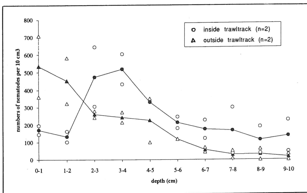
Fig. 3. Mean densities of nematodes ( n \times 10 \text{ cm}^{-3} ) in sediment samples taken inside ( n=2 ) and outside ( n=2 ) the track of a 12-m beam trawl, 17 hours after trawling (April study) (data NIOO-CEMO). Open symbols denote the measured values, black symbols denote mean values.
