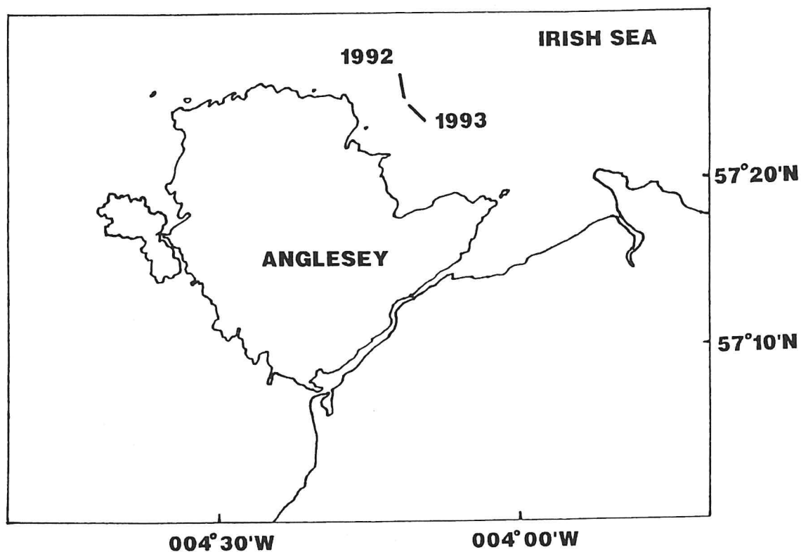
Fig. 1. The location of the study area in the Irish Sea off the north Wales coast and the position of the 4-m beam trawl tows made in August 1992 and April 1993.
