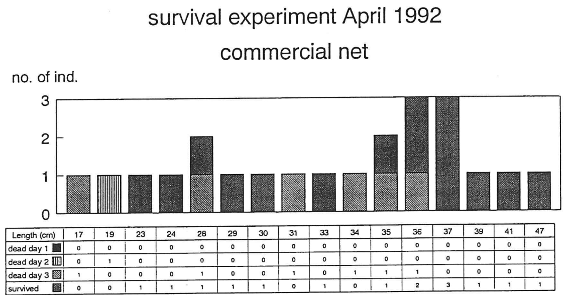
Figure 3. Length-frequency distribution of plaice used in the survival experiments in April 1992 and March 1993. The number of animals brought dead aboard (March 1993 experiment) and dead at day 1, 2 and 3 of the experiment are indicated.
