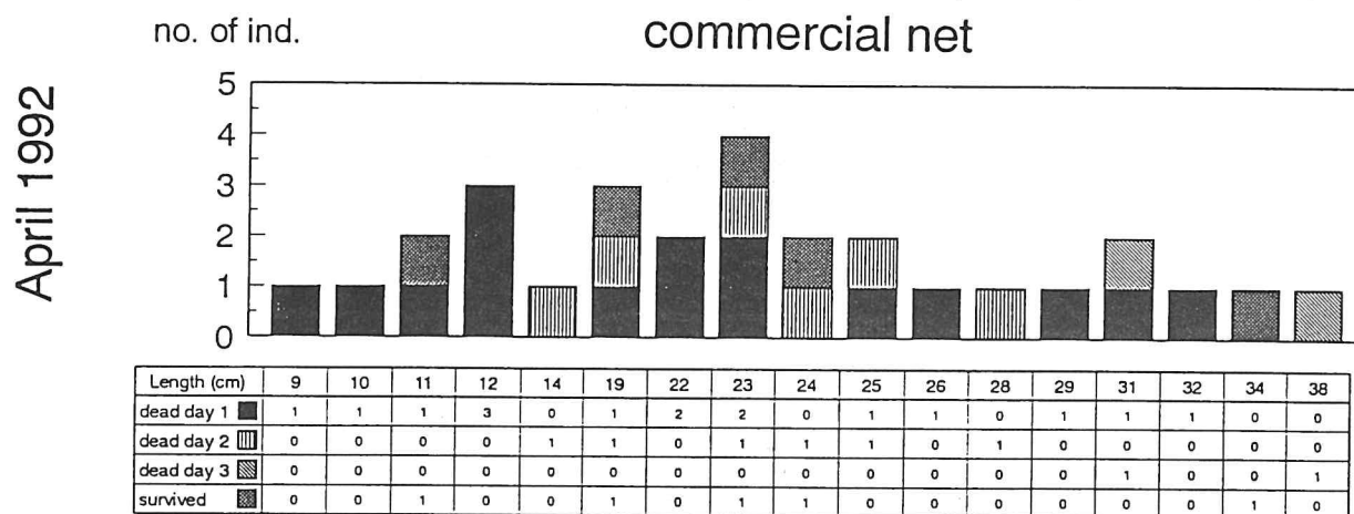
Figure 3. Length-frequency distribution of sole used in the survival experiments in April 1992 and March 1993. The number of animals brought dead aboard (March 1993 experiment) and dead at day 1, 2 and 3 of the experiment are indicated.
