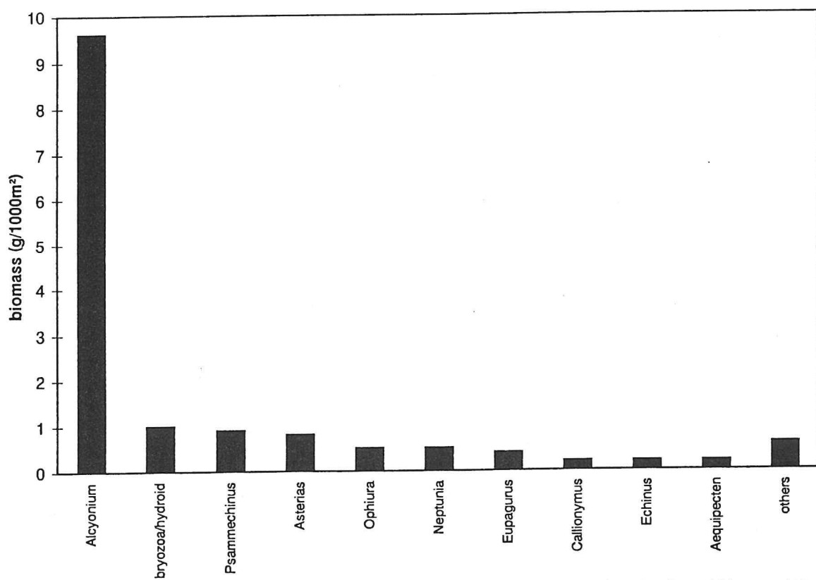
Fig. 1. The ten dominant species in the benthic community at the experimental site, based on density and biomass. NB. A. digitatum and bryozoans/hydroids have been omitted from the density analysis because of the difficulty of quantifying individuals or colonies.
