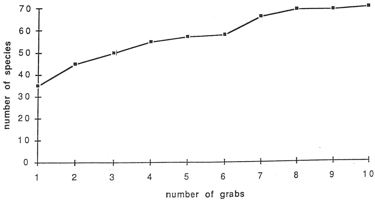
Fig. 6. Cumulative species number in the IMPACT box, based on 10 grabs at station VH 96.
