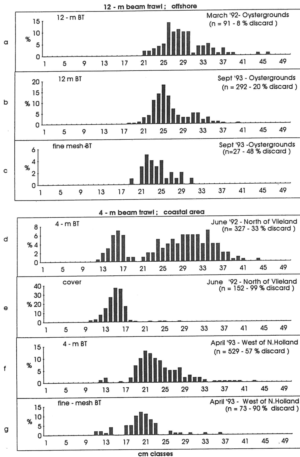
Figure 4. The length frequency distribution of sole ( Solea solea ). Catches with 12-m beam trawls (12mBT) offshore (a,b) and 4-m beam trawls (4mBT) in coastal areas (d,f) compared with catches in fine-meshed cod-end covering net (cover,e) or fine-meshed trawl (c,g).
