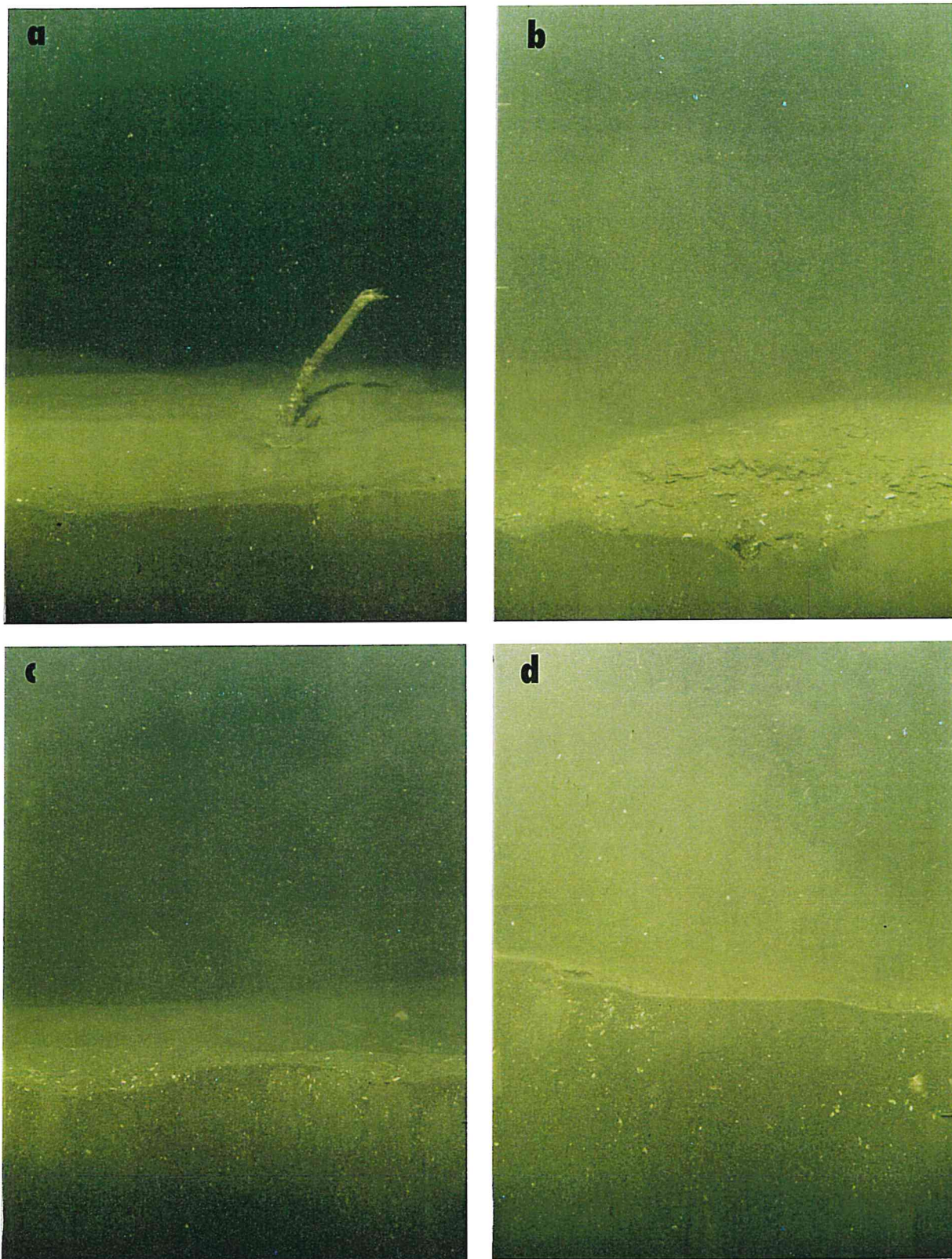
Fig. 9a-d. REMOTS sediment profile photographs taken in heavily trawled German IMPACT box. a) ripped off Lanice tube b) eroded internal sediment layers c) sediment inhomogenities d) sediment inhomogenities
