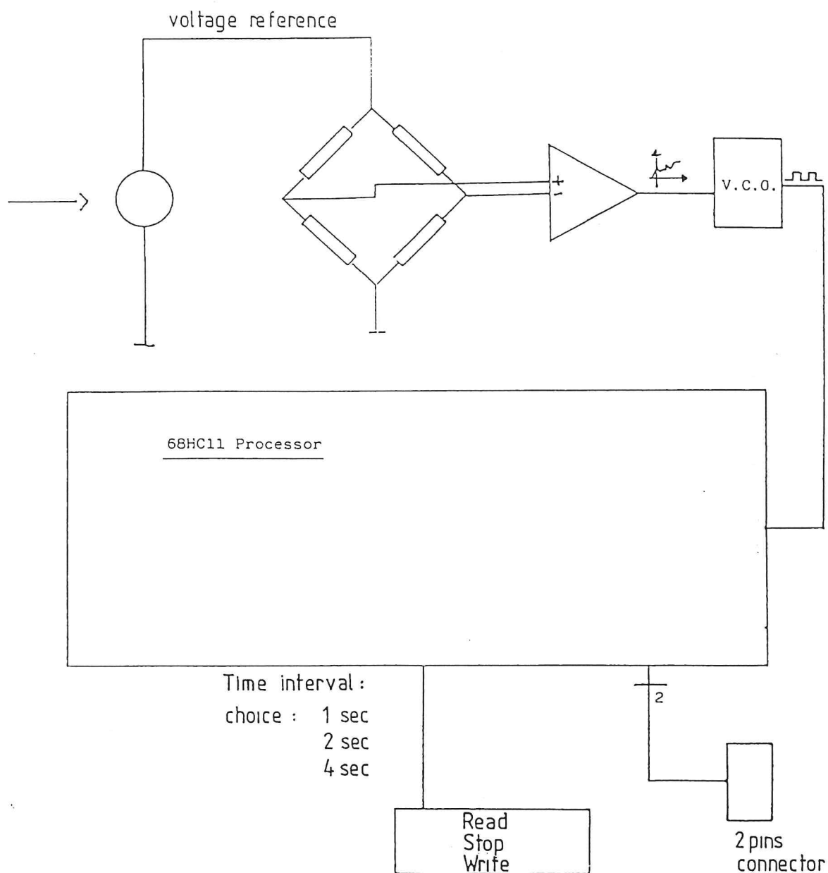
Fig. 1. Measuring principle.
