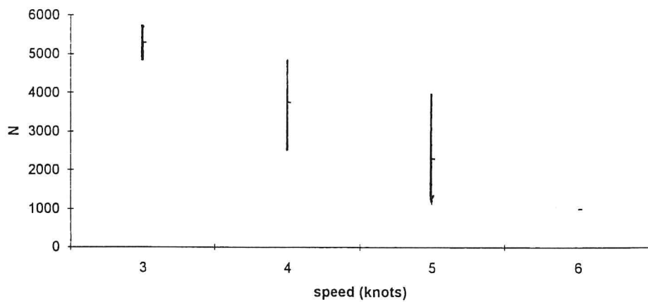
Fig. 18. Pressure force limits.
