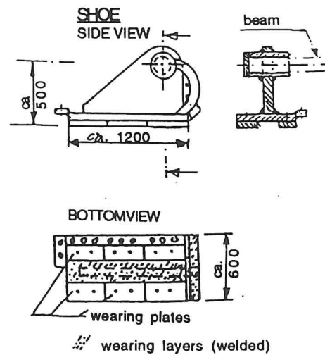
Fig. 3b. Gear-detail
