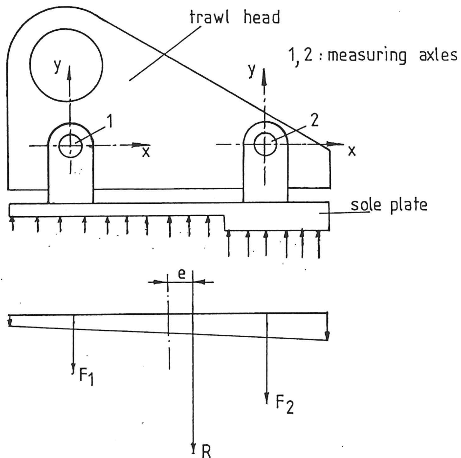
Fig. 3. Instrumented trawlhead-principle.
