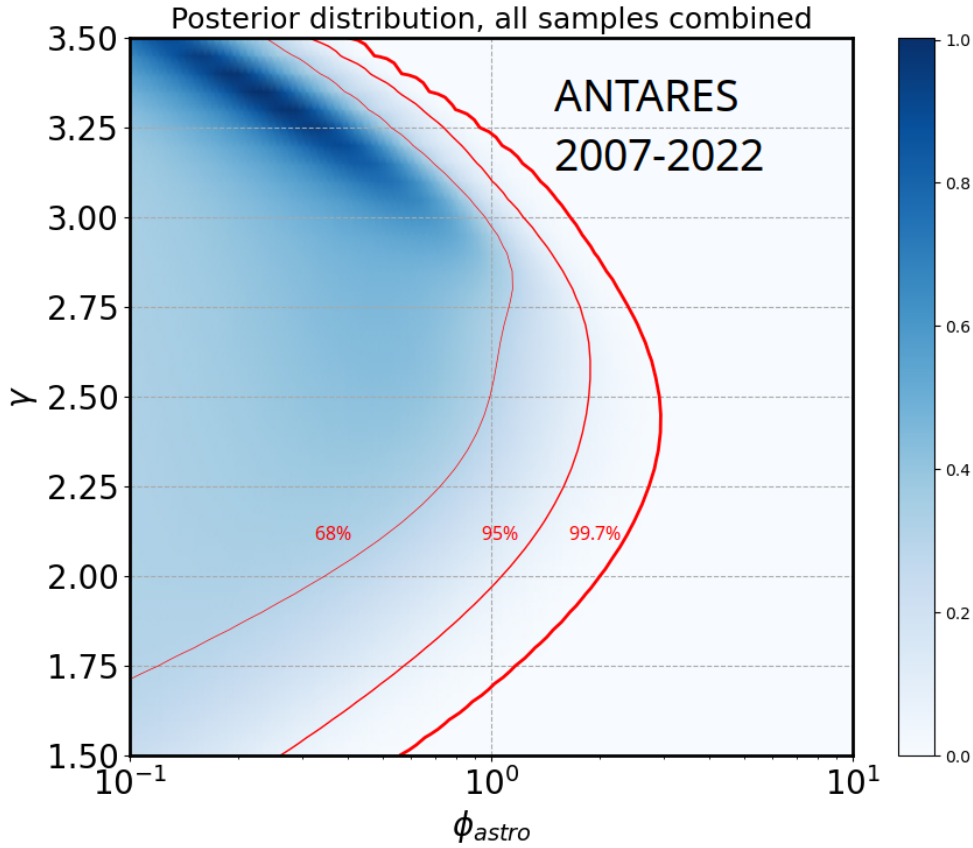
Figure 4. Posterior probability distribution (see equation (3.2)) in the 2D (\phi_{\text{astro}}, \gamma) phase space from the fit of all ANTARES samples combined together. The colour scale shows the posterior probability upscaled so that the maximum is set to 1. The three red lines show (from thinnest to thickest) the 68%, 95%, and 99.7% posterior probability credible area.
