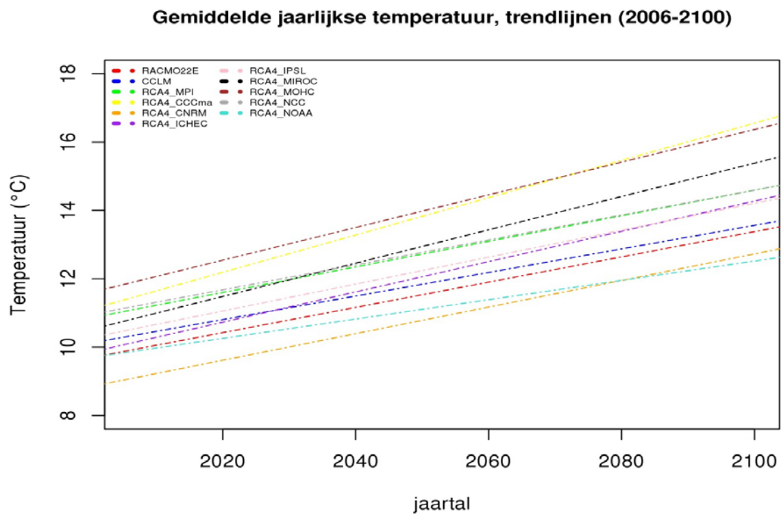
Figure 5: Mean yearly temperature 2006-2100 (RCP8.5), trend lines
