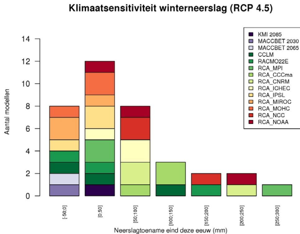
Figure 20: Change in winter precipitation for Uccle by the end of the century (RCP4.5)
