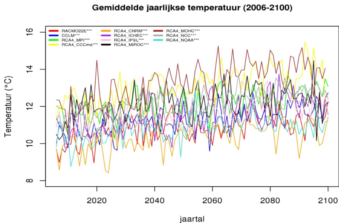
Figure 2: Mean yearly temperature 2006-2100 (RCP4.5)
