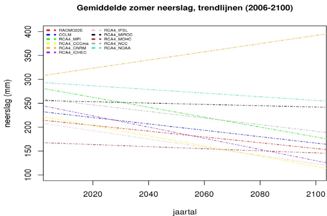
Figure 13: Mean summer precipitation 2006-2100 (RCP8.5), trend lines
