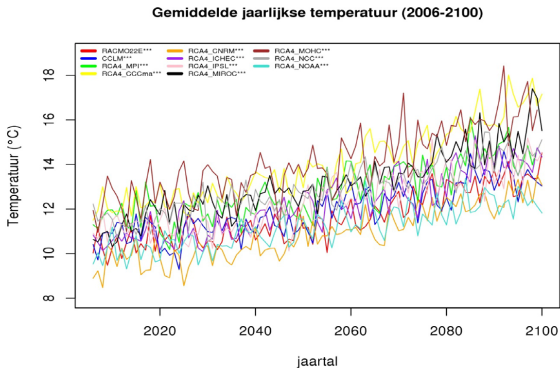
Figure 4: Mean yearly temperature 2006-2100 (RCP8.5)
