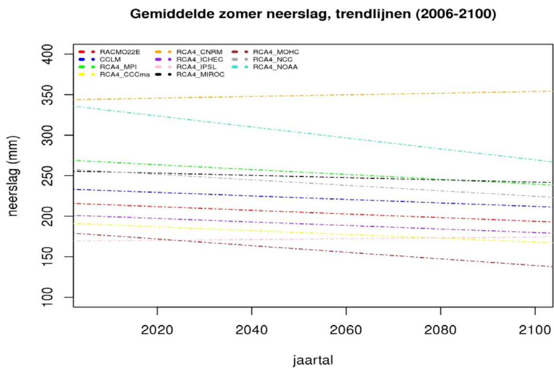
Figure 11: Mean summer precipitation 2006-2100 (RCP4.5), trend lines
