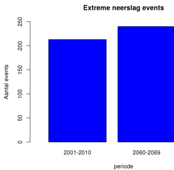
Figure 28: Number of extreme precipitation events for two periods (2001-2010 and 2060-2069)
