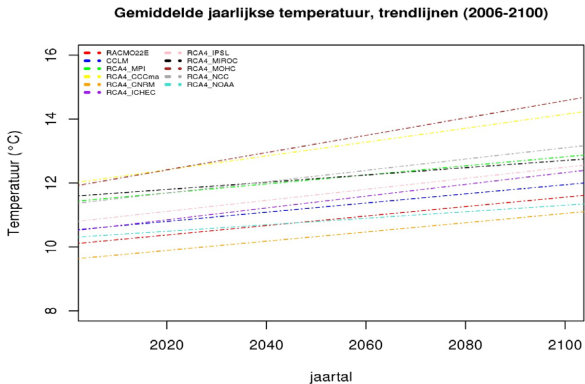
Figure 3: Mean yearly temperature 2006-2100 (RCP4.5), trend lines
