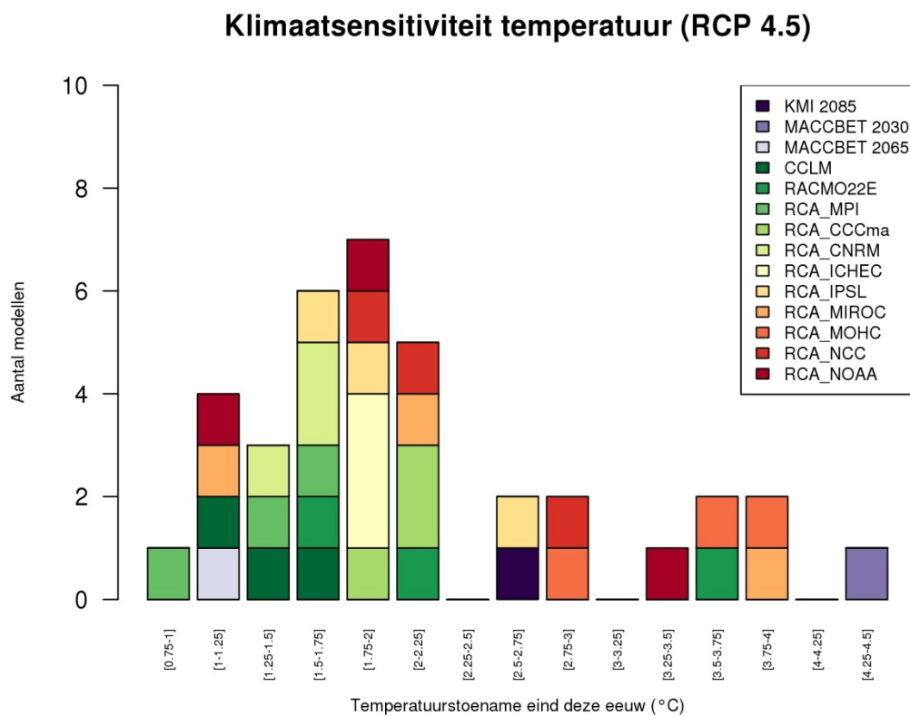
Figure 17: Temperature increase for Uccle by the end of the century (RCP4.5)
