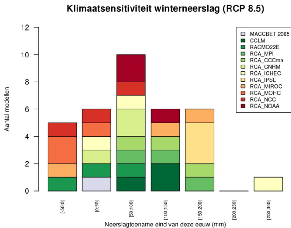
Figure 21: Change in winter precipitation for Uccle by the end of the century (RCP8.5)
