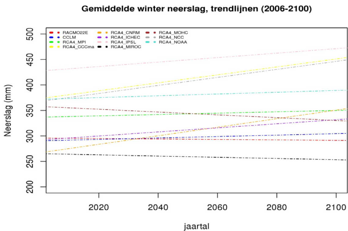
Figure 7: Mean winter precipitation 2006-2100 (RCP4.5), trend lines
