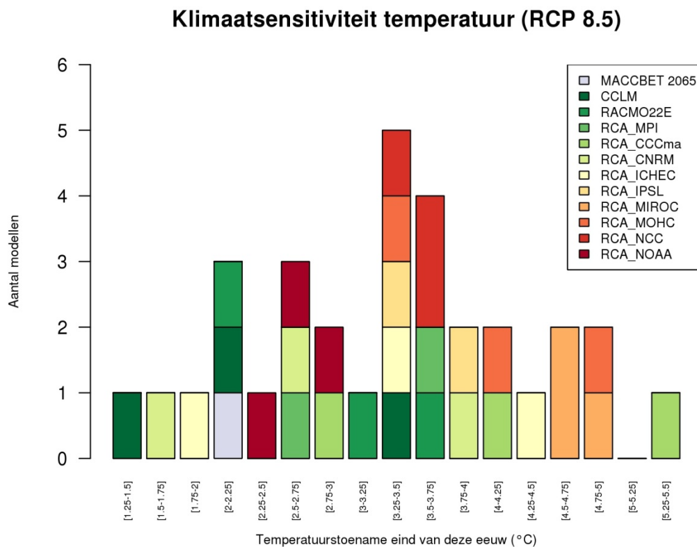
Figure 18: Temperature increase for Uccle by the end of the century (RCP8.5)
