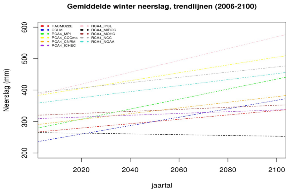
Figure 9: Mean winter precipitation 2006-2100 (RCP8.5), trend lines
