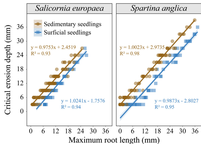
Fig. 4. The critical erosion depth (methods cf. Fig. 1b), required for the dislodgement of seedlings that can resist the maximum BSS applied in the flume, as a function of the maximum root length under two establishment scenarios: without (blue; surficial seedlings) and with (brown; sedimentary seedlings) 5 mm of sediment burial.
